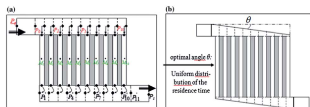
Fig. 12 Schematic representation of the Tzedakis et al. microstructured electrode incorporating 10 microchannels (length 5 mm and depth 50 μm for microchannels and collecting/distributing channels; widths 250 μm for microchannels and 1 mm for collecting/distributing channels). (a) One possible non-optimised geometry, (b) optimised geometry achieved by changing the opening angle \theta of the distributing and collecting channels. Reproduced with permission from ref. 43, Springer.
