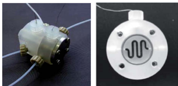
Fig. 6 Photograph of the fixed compact micro-device (left) and its cross-section showing winding channel (right): width 1.5 mm, depth 4 mm, length 57 mm. Reproduced with permission from ref. 31, Wiley.
