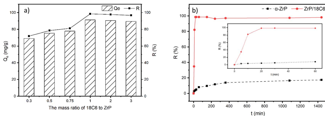
Fig. 6 (a) The effect of mass ratio of 18-crown-ether-6 to zirconium phosphate. (b) Effect of contact time.
