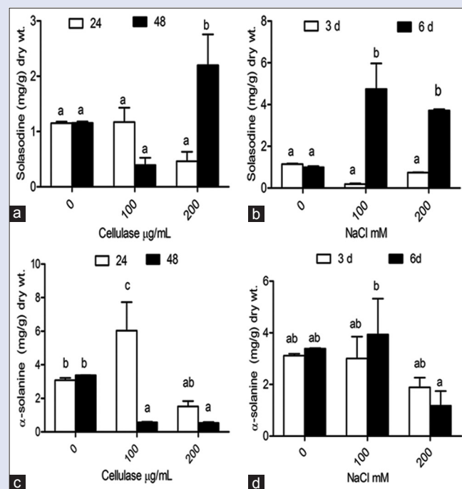
Figure 3: Solasodine and \alpha -solanine content in hairy roots of Solanum khasianum . (a and c) 0 \mu g/mL, 100 \mu g/mL and 200 \mu g/mL concentration of cellulase treatment; (b and d) 0 mM, 100 mM and 200 mM NaCl concentration respectively
