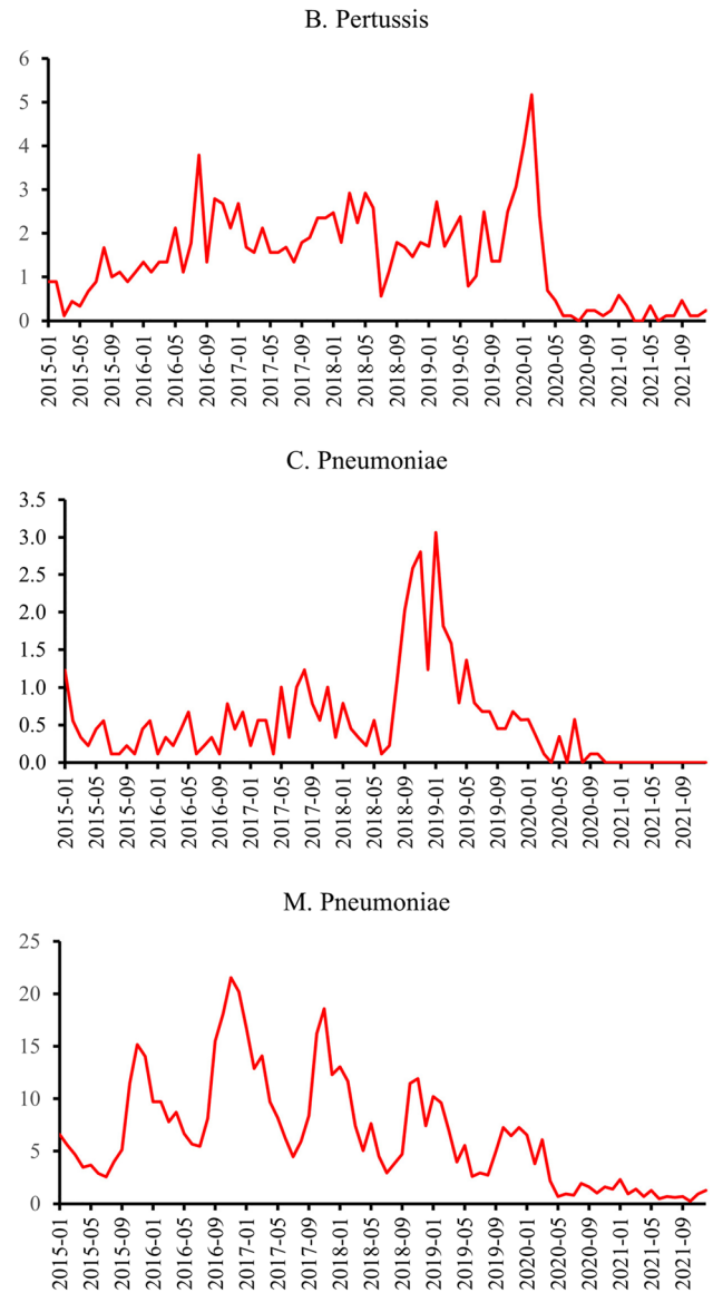
Fig. 1 Monthly incidence per 100,000 of B. pertussis , C. pneumoniae , and M. pneumoniae detections among children aged 0–14 years in Finland from January 2015 to December 2021
