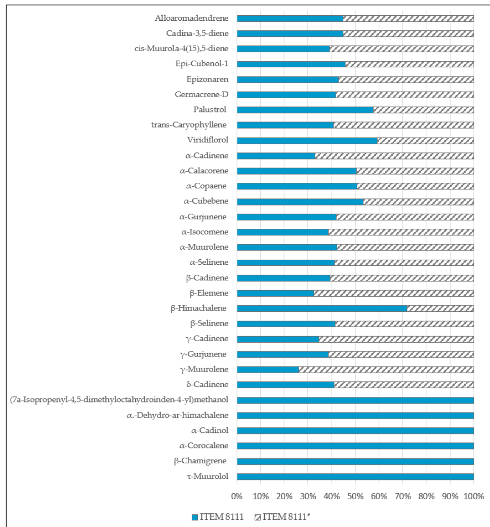
Figure 5. Proportion (%) of terpenes released during day 3 by the toxicigen AFB1-producing (ITEM 8111) and the toxicigen non-AFB1-producing (ITEM 8111*).
