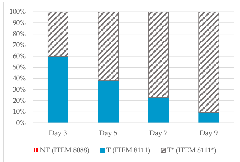
Figure 4. Terpenes distribution between the strains (NT: non-toxicigen strain, T: toxicigen aflatoxin B1 (AFB1)-producing strain, T*: toxicigen non-AFB1-producing strain) emitted of each time point (day 3, 5, 7, 9). The percentage of non-toxicigen (NT) is only present for day 3 and less than 1%, so it is not visible on this graph.
