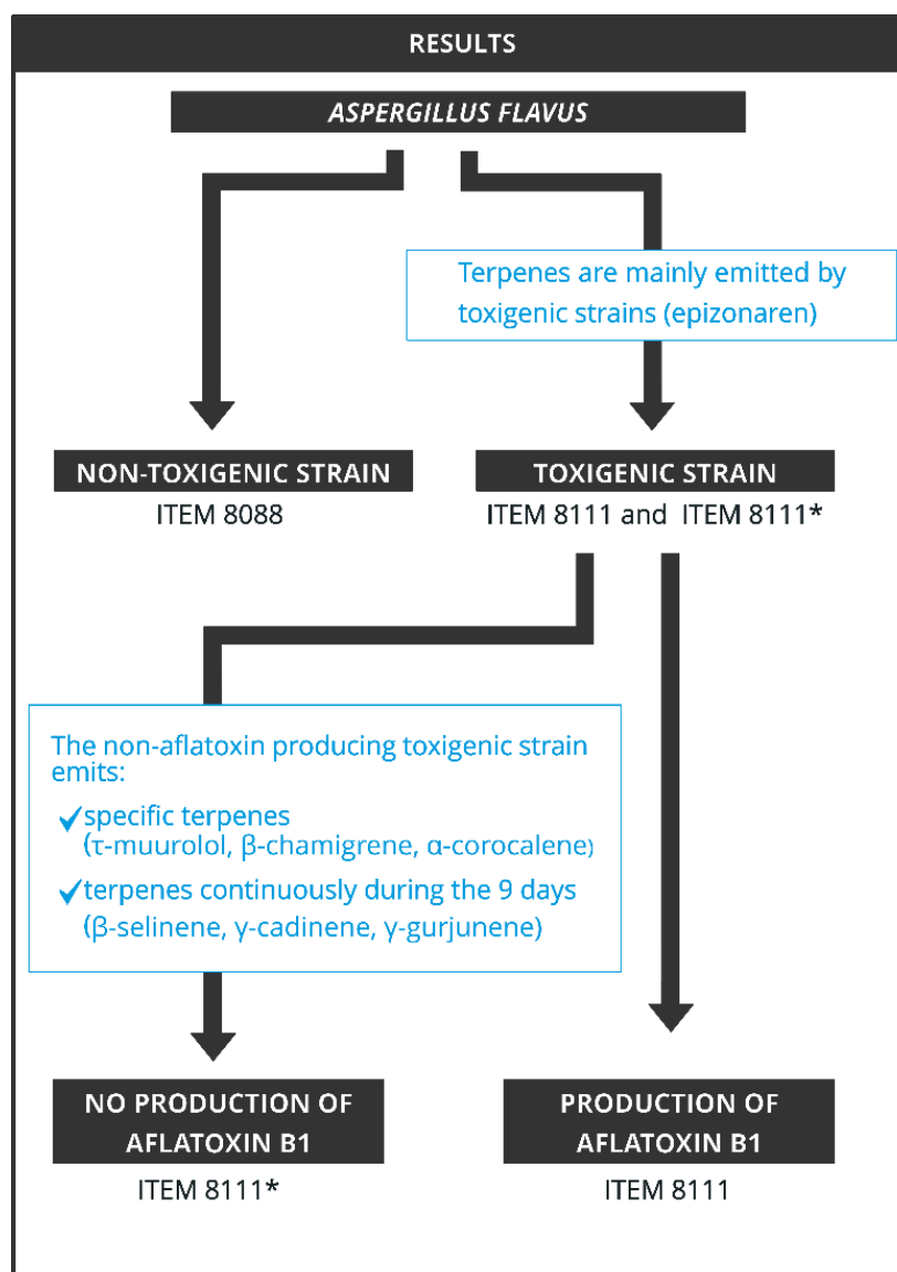
Figure 7. Summary of the results.
