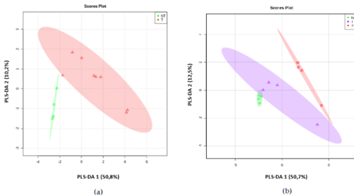
Figure 6. PLSDA (Partial Least Square Analysis) applied on the data (a) of the toxicogenic (T- \Delta ) and non-toxicogenic (NT- \circ ) strains, (b) of the AFB1-producing (T- \Delta ), the non-AFB1-producing (T*- \square ), and non-toxicogenic (NT- \circ ).
