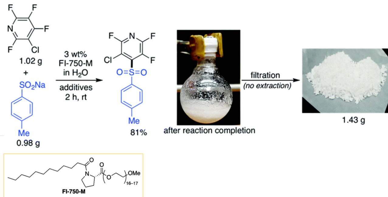
Figure 4. Gram-scale reaction of polyfluoroarene and sodium p -toluenesulfinate salt using FI-750-M micelles. The resulting product was recovered as a solid by filtration, so no organic solvent was required for extraction and purification. Adapted from [71] with permission.
