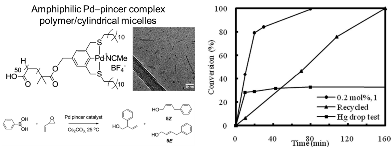
Figure 5. Amphiphilic polymer bearing an SCS pincer palladium complex synthesized by reversible addition fragmentation chain-transfer (RAFT) polymerization. The resulting amphiphile self-assembled into cylindrical (worm-like) micelles in water. The resulting catalyst was used for cross coupling of vinyl epoxide with phenyl boronic acid to afford branched and linear alcohols. The reaction was completed with 0.2 mol% catalyst (100% conversion) after ca. 80 min. Degradation of the catalyst was observed upon recycling of the catalyst and with the addition of Hg(0) (which selectively binds Pd(0)). Adapted from [99] with permission.
