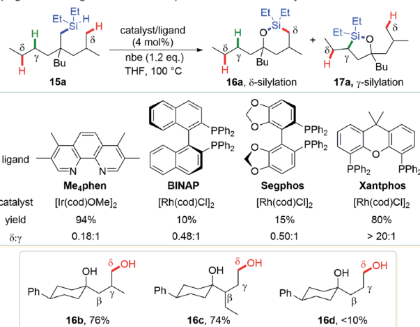
b) Comparison of transition states to explain the \delta -selectivity
