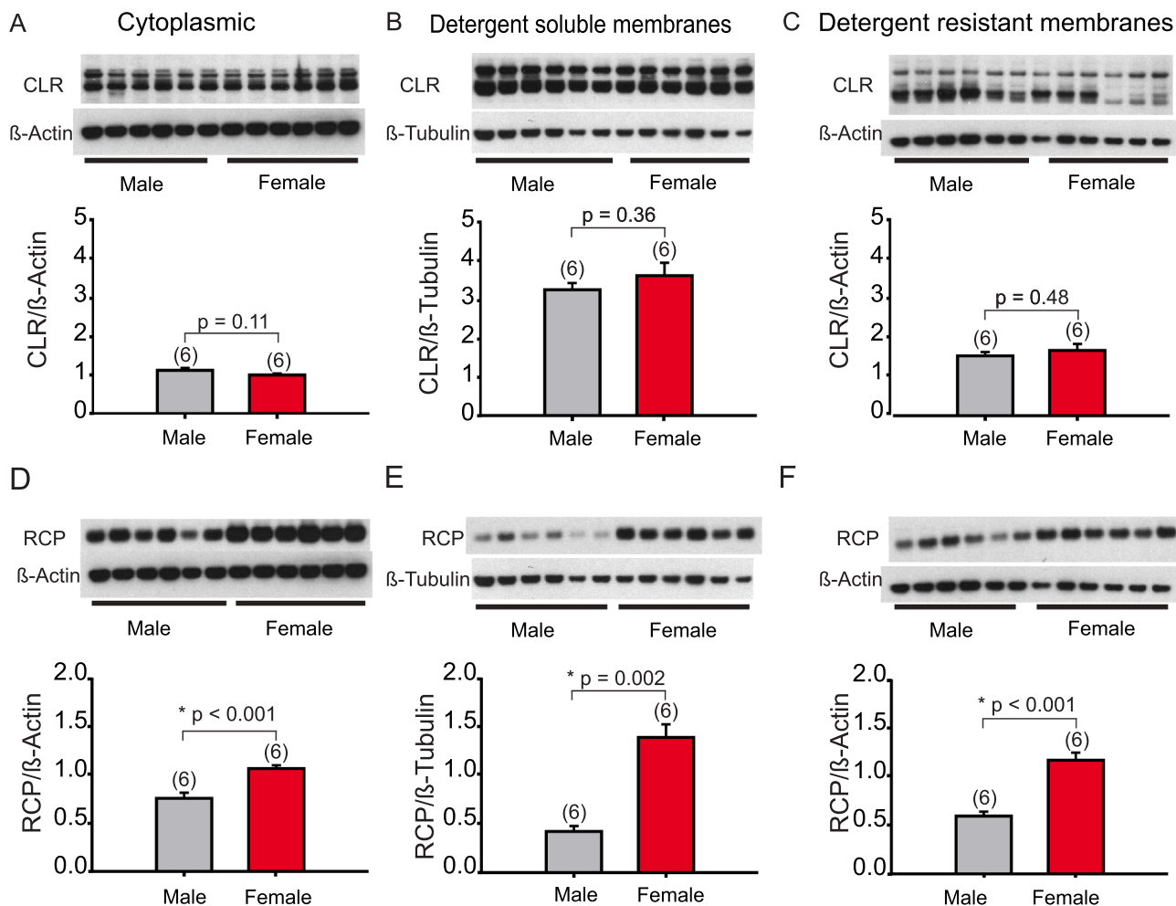
Fig. 1. Distribution of CLR and RCP in the SpVc and upper cervical spinal cord. (A) Western blots of CLR relative to \beta -actin, or \beta -tubulin in female (n = 6) and male (n = 6) rats (control) in cytoplasmic, (B) detergent soluble or (C) detergent resistant fractions of the homogenized tissues. Quantitation of protein levels is shown below each blot. In E–F, the same animals were used to assess changes in the RCP levels in the same fractions. Here and in all figures, error bars = Standard deviations (SD).
