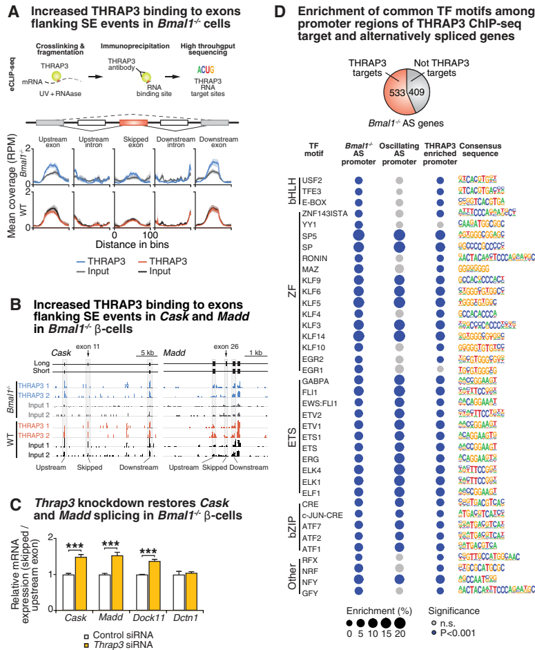
Figure 3. THRAP3 mediates clock-dependent alternative splicing. (A) Schematic of eCLIP sequencing experiment (top) and normalized (reads per million) THRAP3 eCLIP or input sequencing reads along indicated regions of alternatively spliced mRNAs (bottom). Solid line indicates mean for two replicates and shaded area represents 95% confidence interval. (B) UCSC genome browser tracks showing reads from indicated THRAP3 IP and input samples along regions within Cask and Madd RefSeq transcripts. Skipped exons identified by rMATS and flanking exons are shaded in gray and track heights for each sample are standardized to equal height for row shown. (C) Thrap3 siRNA knockdown restores exon inclusion in Bmal1 -/- \beta cells, assessed by qPCR ( n=3 ). (D, top) Pie chart summarizing number of AS genes in Bmal1 -/- \beta cells identified as THRAP3 ChIP-seq targets. (Bottom) Bubble plot indicating enrichment of indicated motifs within promoter regions of AS genes and promoter-localized THRAP3 peaks. Size of bubbles reflects enrichment score for motifs within each indicated set of promoters, and those called as statistically significant (Homer hypergeometric test P < 0.05 ) are shown in blue.
