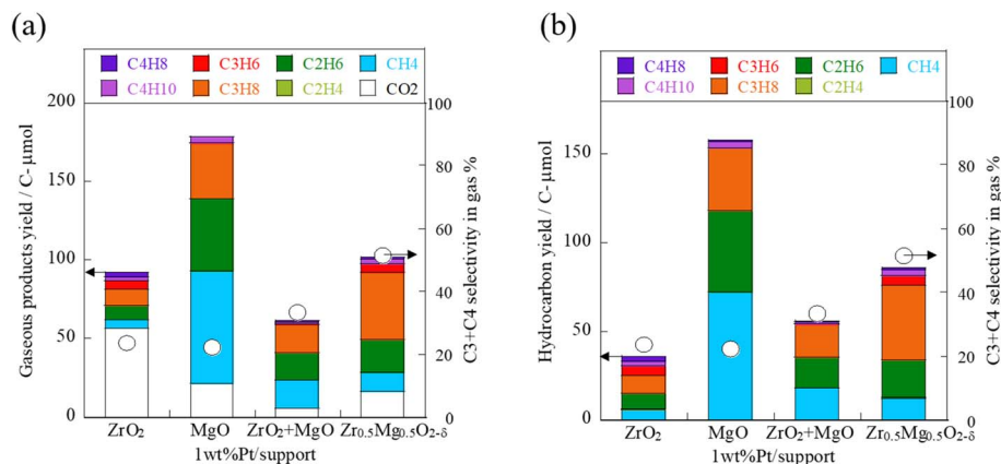
Fig. 4 (a) Gaseous product yield and (b) hydrocarbon yield obtained using 1 wt% Pt/support ( \text{ZrO}_2 , MgO, mixed, doped), cellulose, 443 K, 12 h. Liquid products are shown in Fig. S8 in ESI†
