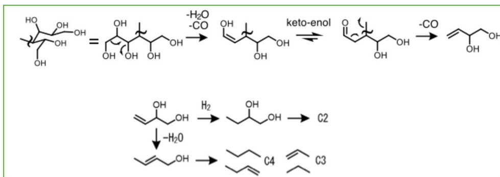
Fig. 11 Estimated reaction mechanisms from cellulose over Pt/Zr 0.5 Mg 0.5 O 2-δ catalyst.
