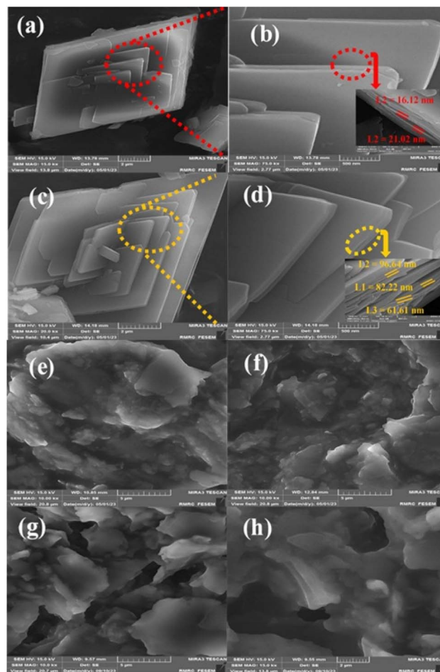
Fig. 2 FE-SEM images with different magnifications of (a and b) Ni-MOF, (c and d) Ni-Bio-MOF, (e) Ni-Bio-MOF/NIP-PL-Met, (f) Ni-Bio-MOF/MIP-PL-Met (before removal of DCF), (g and h) Ni-Bio-MOF/MIP-PL-Met (after removal of DCF).
