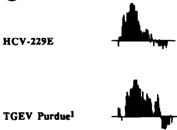
Fig. 4. (A) Comparison of the predicted amino acid sequences of mRNA 5 (ORF5) from HCV-229E (top row), TGEV Purdue ( 1 Rasschaert et al., 1987; middle row) and TGEV Miller ( 2 Wesley et al., 1989; bottom row) aligned for maximum homology. Regions common to the two proteins are underlined and differences with TGEV Miller are indicated on the bottom row. (B) Hydropathicity profiles of the protein encoded by mRNA 5 of HCV-229E and TGEV Purdue determined according to Kyte and Doolittle (1982). The analysis was performed on an Apple Macintosh Plus computer with the MacGene Plus program (Applied Genetic Technology Inc., Fairview Park, OH). Each point is the mean hydropathicity of a span of seven residues. Peaks extending upwards correspond to hydrophobic regions and peaks extending downwards to hydrophilic areas.
