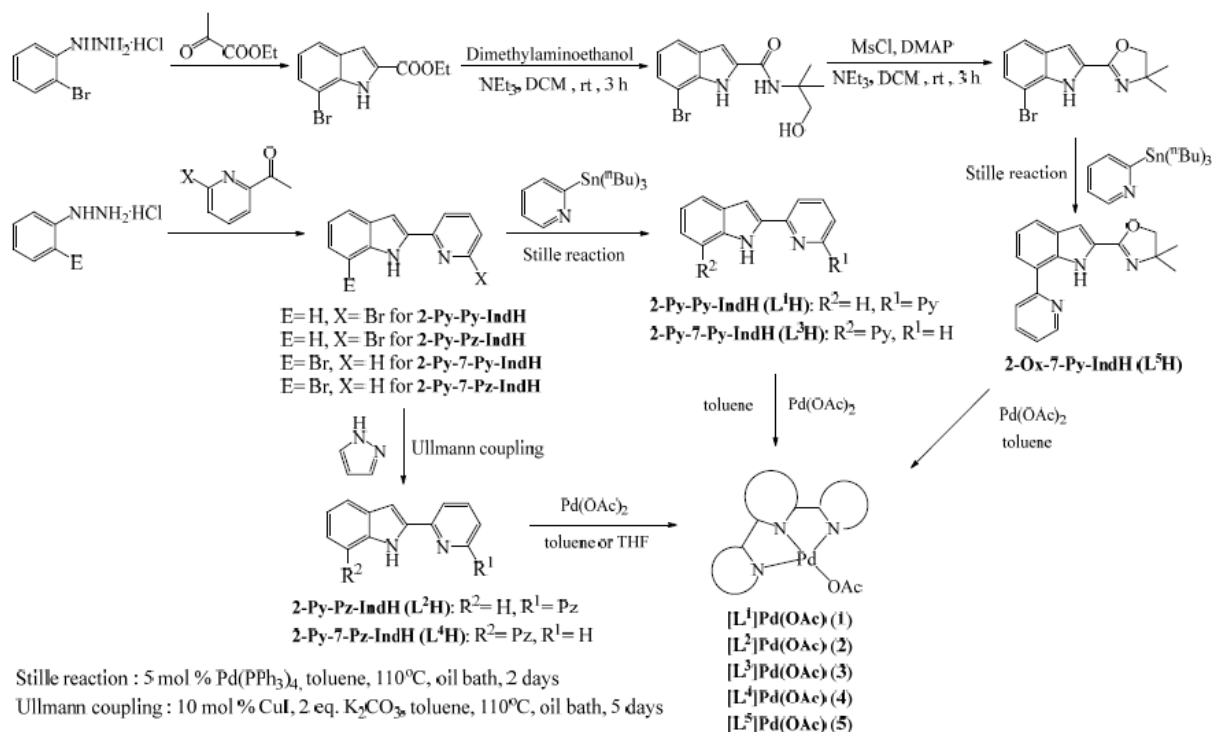
Scheme 1. Preparation of ligand precursors and palladium complexes.
