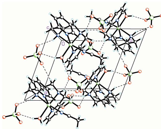
Figure 2 Packing diagram, viewed along the c axis, showing the extensive O—H···O, N—H···O, and C—H···O interactions linking the cations and anions into a complex three-dimensional array. For the disordered moieties, only the major conformation is shown.
