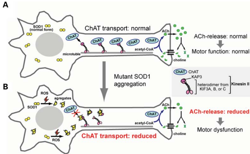
Figure 8. A schematic diagram for a mutant SOD1 toxicity and impairment of axonal transport of ChAT. In healthy motor neurons (A), ChAT is continuously transported by kinesin-2 motor, comprising KIF3A, KIF3B/C and KAP3, toward the neuromuscular junction where ACh functions as a neurotransmitter. ACh is released into the synaptic cleft upon stimulation and rapidly degraded into choline and acetic acid by AChE. Choline is taken up into the nerve terminal by choline transporters and then ChAT synthesizes ACh from choline and acetyl-CoA. The reaction catalyzed by ChAT is the rate-limiting step for ACh supply to the nerve terminals. In motor neurons expressing mutant SOD1 (B), mutant SOD1 proteins were converted into misfolded forms as a result of increased ROS generation and/or reduced proteasomal activity. Certain misfolded species preferentially binds to KAP3 and inhibit the binding of ChAT to KAP3, thereby causing a decrease in ChAT transport. This decrease in ChAT in the nerve terminals can constitute a mechanism that causes motor dysfunction.
