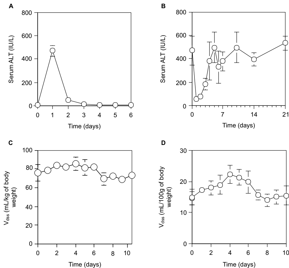
Figure 2 Time course of physiological effects of drugs in rats during liver regeneration after 70% PH.
