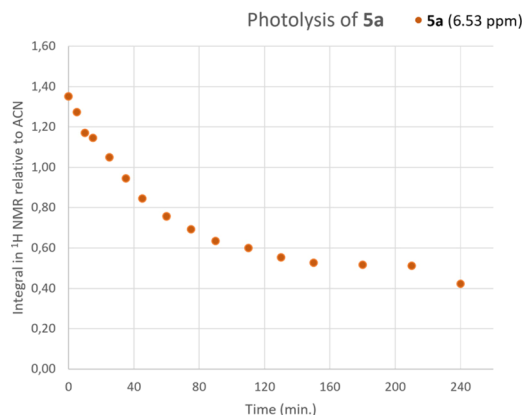
Figure 4. Rate of decomposition for compound 5a upon irradiation in an NMR tube. The ^1\text{H} -NMR signals due to residual proton(s) in the solvent (acetonitrile) were used as an internal standard.
