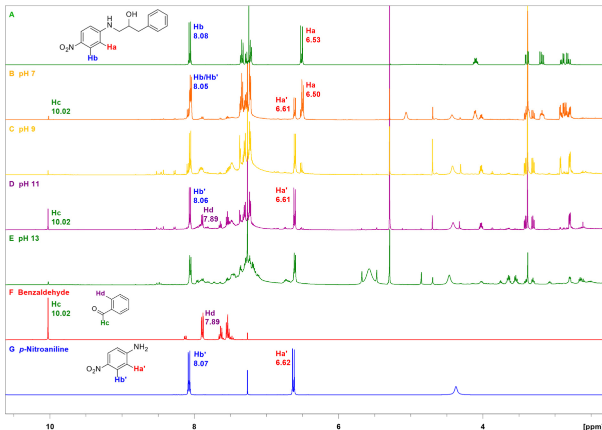
Figure 3. ^1\text{H} -NMR spectra of the photolysate from compound 5a irradiated at pH from 7 to 13 for 2 h and reference spectra of benzaldehyde and p -nitroaniline.
