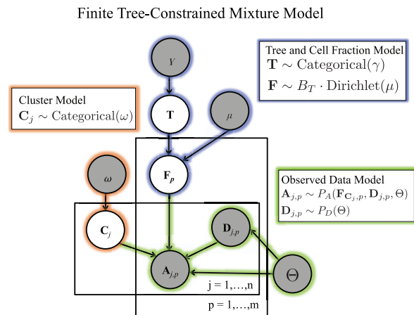
Fig. 2. Generative model for variant allele counts A from DNA sequencing data of a tumor. A latent (unobserved) clone tree T generates m samples, each consisting of mixtures of cells with different mutations. Each mutation is assigned to a cluster C_j . A cluster i of mutations occur in fraction F_{i,p} of cells in sample p . Variant read counts A are generated for each mutation with a binomial likelihood model, given an observed total read counts D
