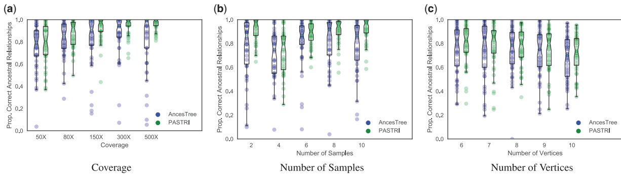
Fig. 6. The effect of coverage, number of samples, and number of vertices on performance of AncesTree and PASTRI. For every combination of parameters, we generate 50 trees. Here we report the proportion of ancestral relationships that were correctly recovered. Overall, PASTRI has higher average performance for all sets of parameters, but the magnitude of this effect differs. (a) As the coverage increases, and uncertainty in variant allele frequencies decreases, PASTRI's accuracy increases. AncesTree's accuracy increases initially, but declines at the highest coverages. (b) Similarly, as the number of samples increases and the problem becomes more constrained, PASTRI's accuracy increases, while AncesTree's accuracy peaks with four samples, and then declines. (c) As the number of vertices in the tree increase, both AncesTree and PASTRI see a similar moderate decline in performance, although PASTRI consistently outperforms AncesTree
