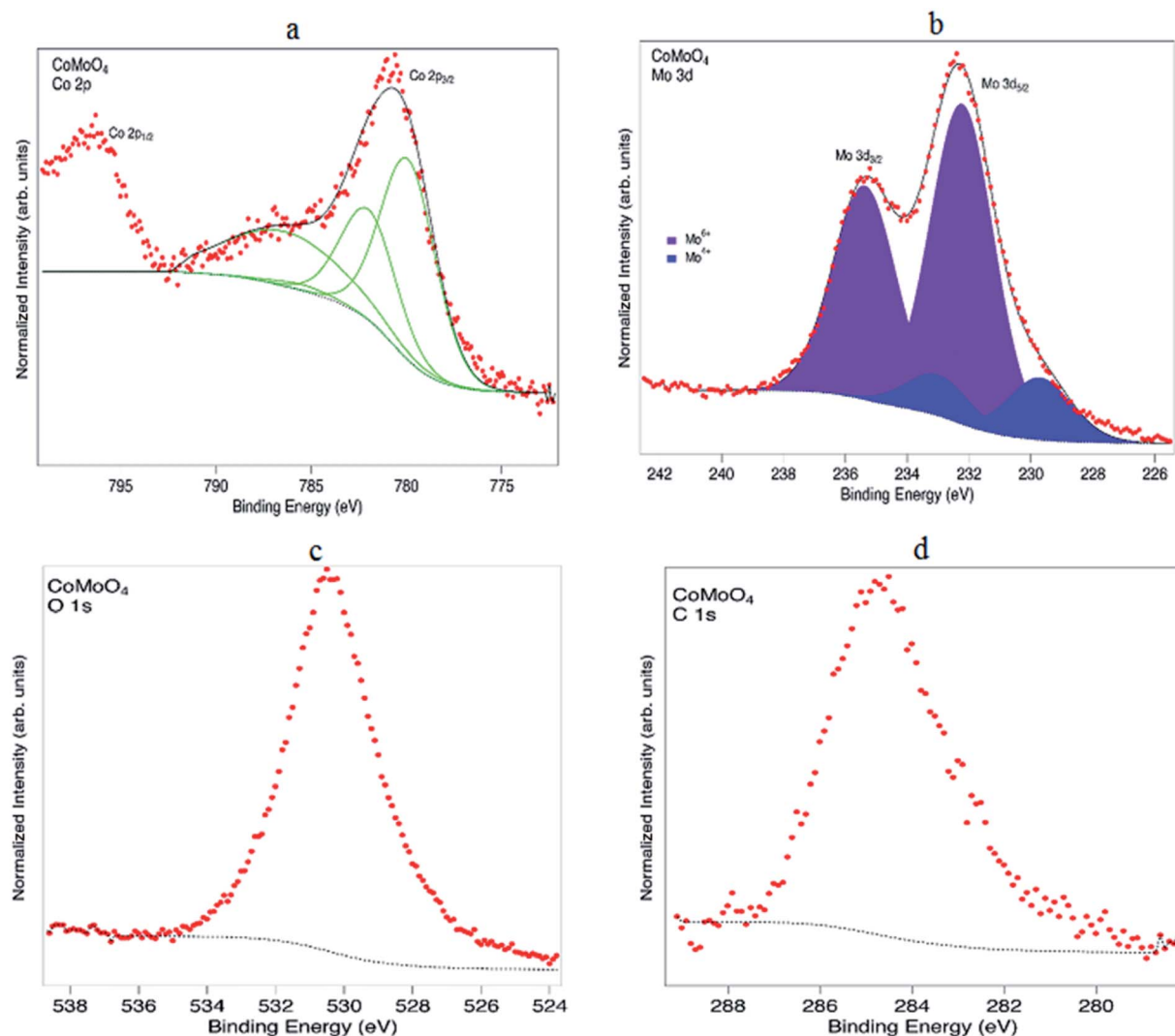
Fig. 5 (a) XPS spectra of Co 2p recorded from CoMoO 4 , (b) spectra of Mo 3d, (c) XPS spectrum of O 1s and (d) spectrum of C 1s of CoMoO 4 .
