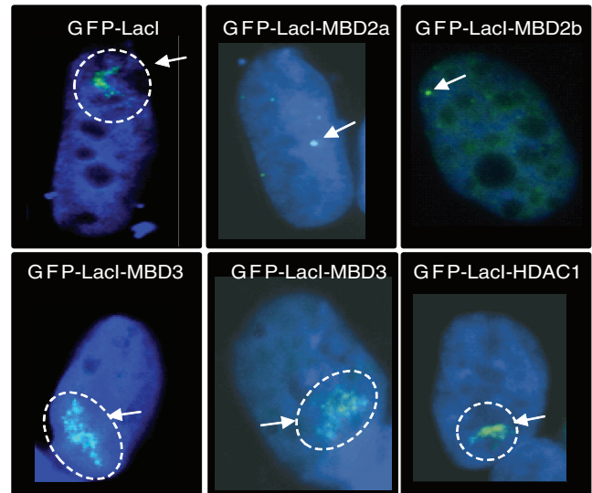
Figure 2. In contrast to MBD3 and to other NuRD components, LacI-MBD2a or LacI-MBD2b dramatically compact the euchromatic LacO array. RREB1 cells were transfected with GFP-LacI, GFP-LacI-MBD2a/b, GFP-LacI-MBD3 and GFP-LacI-HDAC1 as indicated. Samples were visualized for DNA (blue) and GFP (green). The arrows point to the compact array or to the expanded array (dotted circle).
