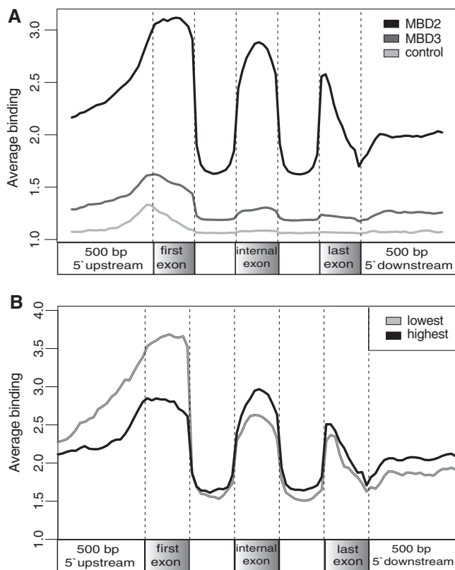
Figure 8. MBD2 specifically marks exon sequences. (A) MBD2 and MBD3 occupancy plotted as average of all sequencing reads across the following intervals: 500 bp upstream, first exon, all internal exons compiled as a single exon, last exon and 500 bp downstream according to their relative positions within the transcripts. First exon, internal exons and last exon were partitioned into 10 bins. 500 bp upstream and 500 bp downstream were partitioned into 20 bins. (B) MBD2 binding in respect to its association with low (inactive) and highly expressed genes (active). Highly expressed genes have lower MBD2 binding in the promoter in contrast to higher binding across internal exons.
