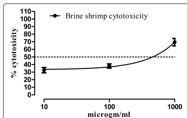
Figure 3 Brine shrimp cytotoxicity of crude methanol extract of Tylophora hirsuta .
