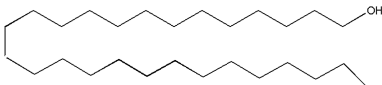
Figure 2 Structural formula for Heptaacosanol isolated from Tylophora hirsuta .
