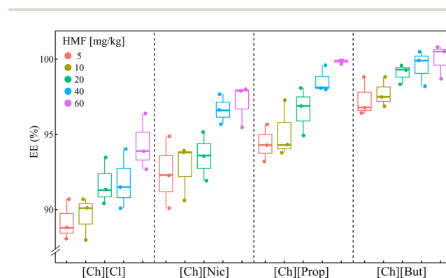
Fig. 3 Extraction efficiency (EE, %) using the aqueous biphasic systems composed of choline-based ILs.
