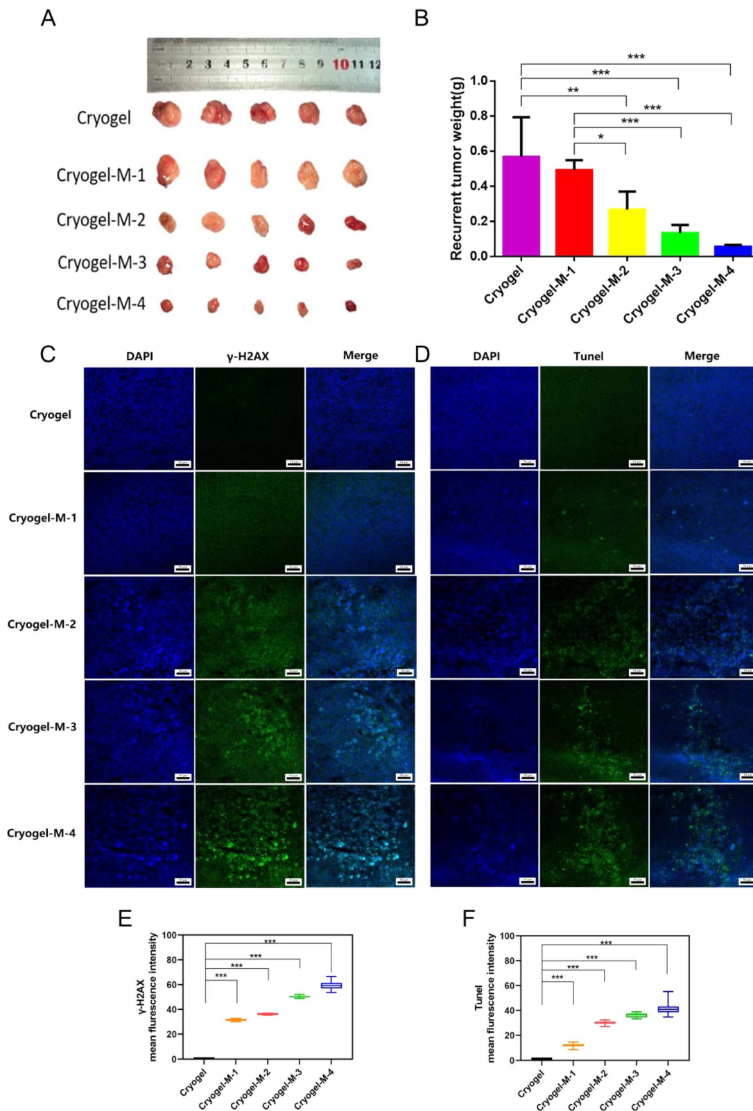
Fig. 5 (A) Excised recurrent solid tumors from different treatment groups on the 30th day. (B) Tumor weight statistics chart ( n = 5 ). (C) \gamma -H2AX analysis of excised recurrent tumor on the 30th day. (D) TUNEL analysis of excised recurrent tumor on the 30th day. Scale bar = 50 \mu m. (E) Mean fluorescence intensity of \gamma -H2AX ( n = 5 ). (F) Mean fluorescence intensity of TUNEL ( n = 5 ).
