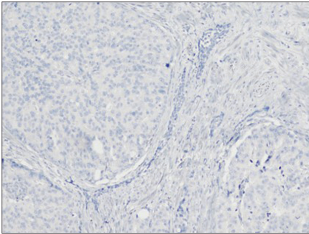
Figure 5: ERG/EZH2
