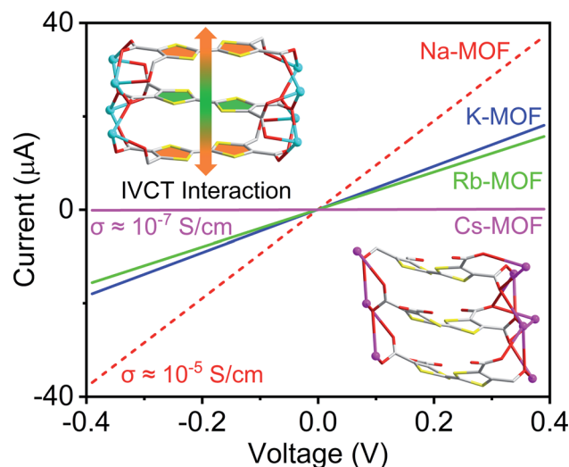
Fig. 1 A representation of how \pi - \pi -distance, TTFTC •+ population, and ICVT interactions between the mixed valent TTFTC ligands in MOFs affected their electrical conductivity.
