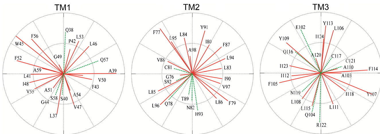
Figure 3. Polar plots representing the SASA values ( \text{\AA}^2 ) and the relative orientation of all the residues that form a part of the three TM domains (hydrophilic and hydrophobic residues are given in green and red, respectively).
