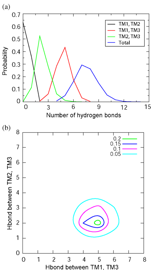
Figure 6. (a) Probability distribution of the number of hydrogen bonds between each pair of TM domains in bundle 2. (b) Contour plot of the probability distribution of the number of hydrogen bonds between TM1 and TM3, and TM2 and TM3.
