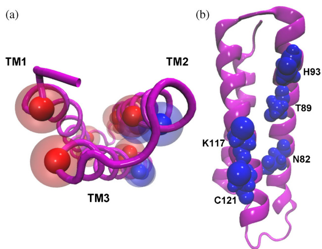
Figure 9. Structure of bundle 2 after the simulation. (a) Top view. (b) Side view. Interfacial hydrophilic residues between TM domains are presented as red spheres, and hydrophilic residues which are present outside the bundle and form a hydrophilic stripe, are shown as blue spheres.
