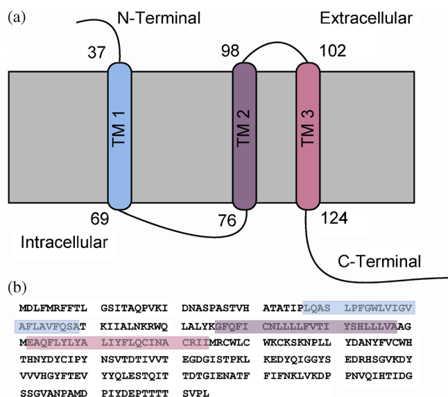
Figure 1. (a) Schematic representation of the three transmembrane domains of SARS 3a. (b) Sequence of the SARS 3a protein. Residues that are part of TM1, TM2 and TM3 are highlighted using similar colors in (a).
