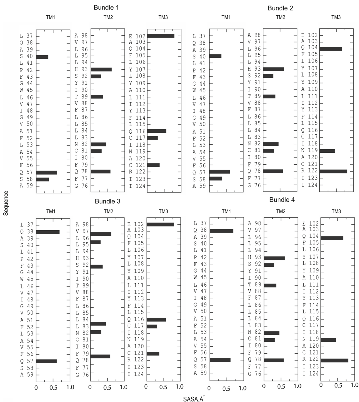
Figure 5. Sequence versus SASA of the overlapping hydrophilic residues in the four potential bundles.
