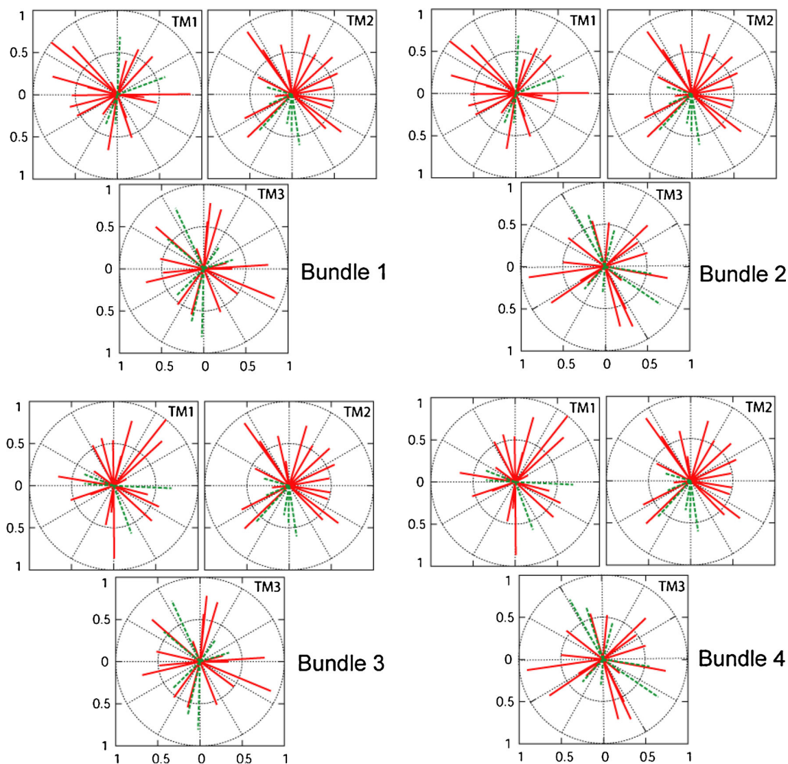
Figure 4. Arrangement of the individual polar plots (figure 3) to form four potential TM domain bundles (1, 2, 3, and 4) with respect to varying orientation of residues.
