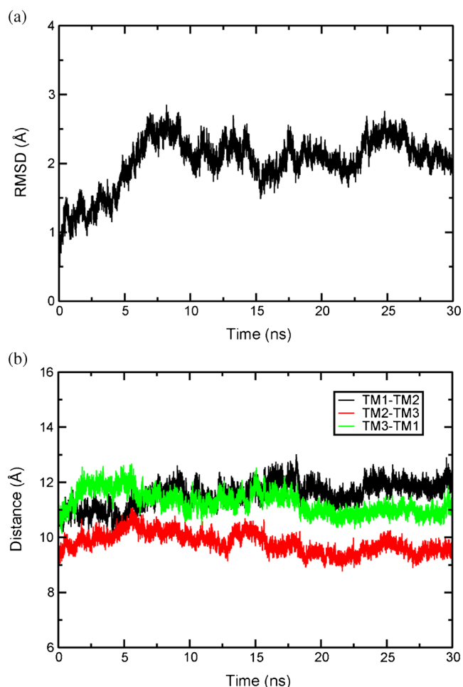
Figure 8. (a) Backbone RMSD of the bundle over the course of equilibration in an explicit membrane environment. (b) Distance between the centers of mass of the three TM domains during the simulation.
