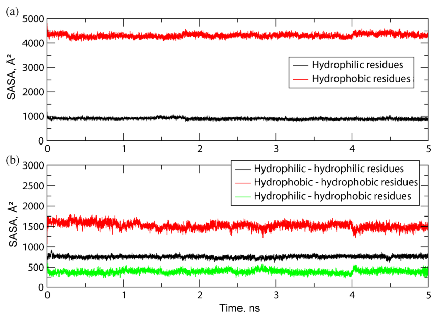
Figure 7. (a) SASA of hydrophilic and hydrophobic residues of bundle 2 against simulation time. (b) Contact area between hydrophilic and hydrophilic residues, hydrophobic and hydrophobic residues, and hydrophobic and hydrophilic residues versus simulation time in bundle 2.
