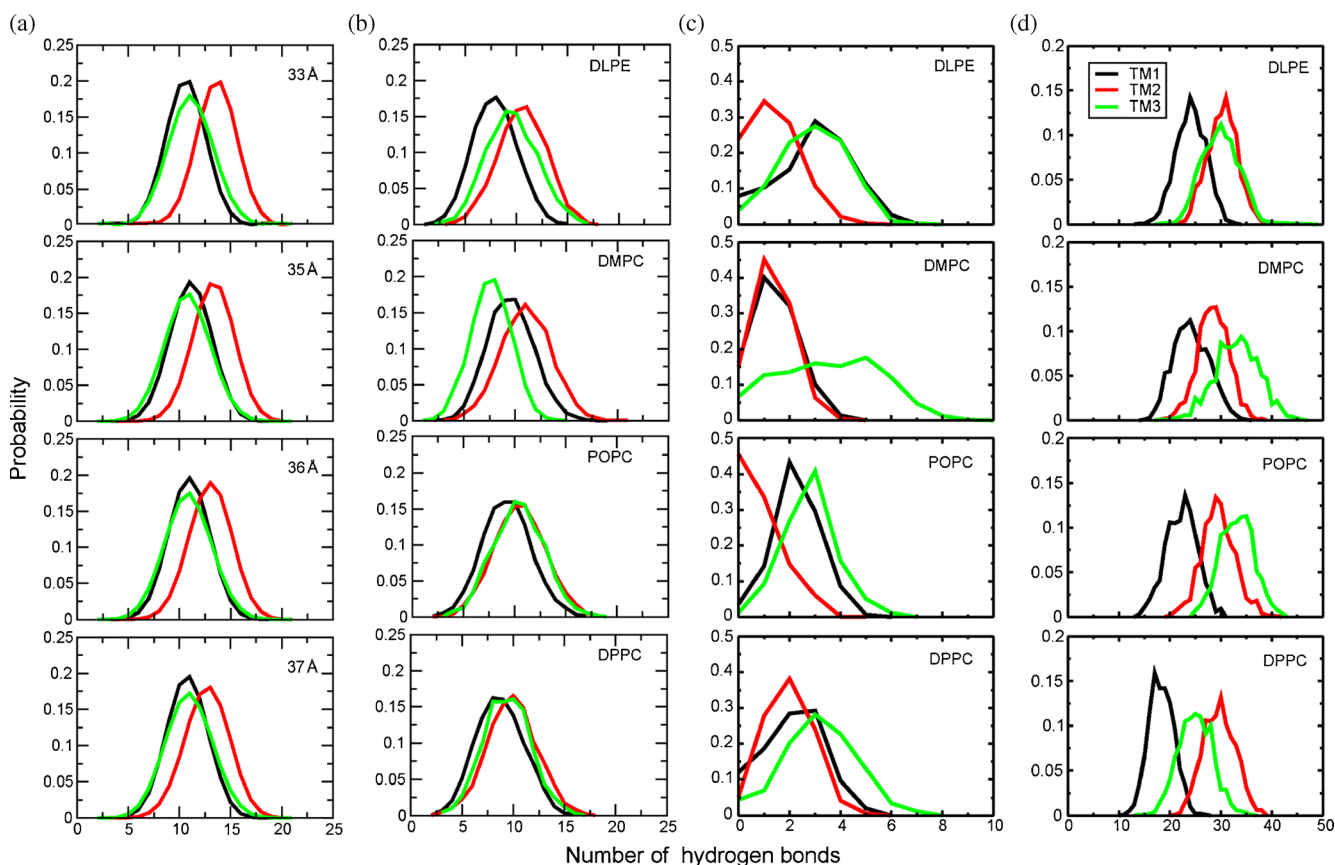
Figure 2. (a) Probability distribution of intra-helical hydrogen bonds of TM domains in implicit membrane simulations. (b) Probability distribution of intra-helical hydrogen bonds of TM domains in explicit membrane simulations. (c) Probability distribution of the number of hydrogen bonds between TM domains and lipid molecules in the explicit membrane simulations. (d) Probability distribution of the number of hydrogen bonds between TM domains and water molecules in the explicit membrane simulations.
