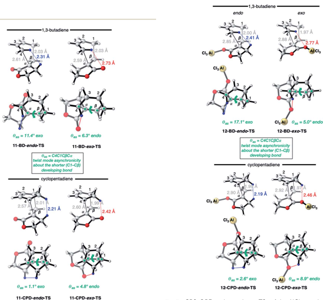
Fig. 6 CBS-QB3 endo - and exo -TSs of the uncatalyzed DA reaction of \alpha -methylene \gamma -butyrolactone 11 with BD and CPD, highlighting key destabilizing close contacts, and the direction and magnitude of twist-mode asynchronicity. Top row: perspective view; bottom row: view down the forming C–C bonds, from the diene side of the TS.
