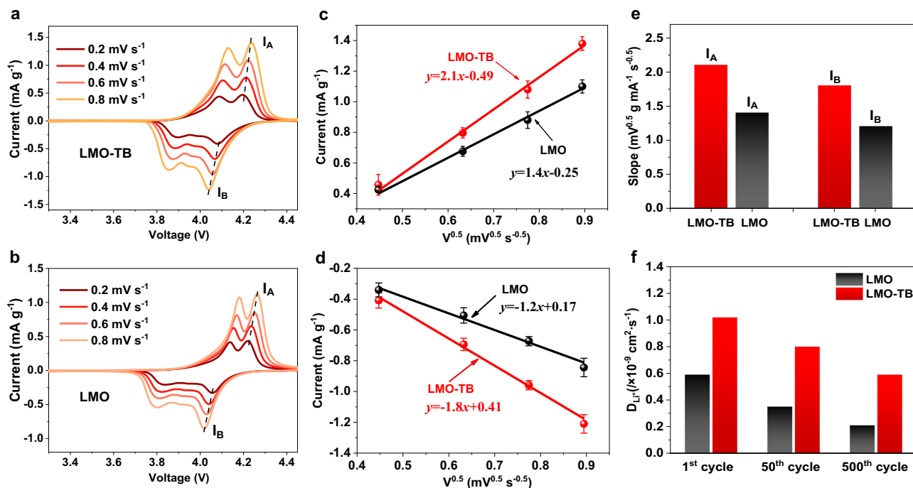
Fig. 5 Lithium-ion diffusion rate of the LMO and LMO-TB cathodes. a, b CV curves at different rates, c, d linear relationship between the major c oxidation ( I_A ) and d reduction ( I_B ) peaks and scan rates. Error bars represent the standard deviations of the value for oxidation and reduction peaks in CV curves, e compared slope values of I_A and I_B , f lithium-ion diffusion coefficients at different cycle numbers.
