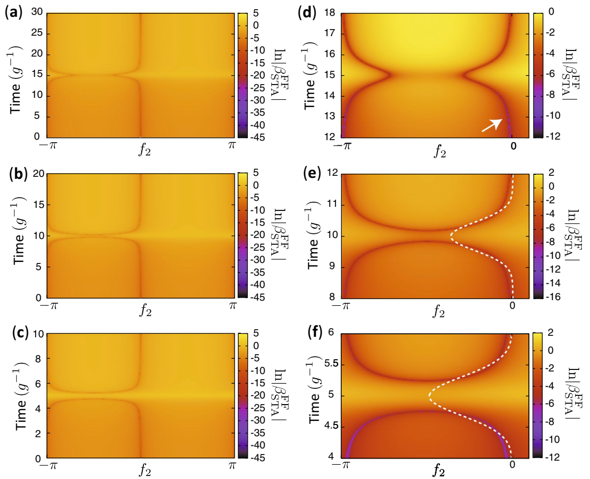
Figure 3. Inter-trajectory travel for shortcuts to adiabaticity. (a–c) \ln|\beta_{STA}^{FF}| as a function of f_2 and t . (a–c) are for T_F = 30g^{-1}, 20g^{-1} and 10g^{-1} , respectively. (d–f) are the closeups of panels (a–c) respectively. The arrow in (d) indicates the speed-controlled trajectory. The white dashed curve in panels (e,f) shows a virtual trajectory. \Delta\omega_0 = 30g , where g is constant.
