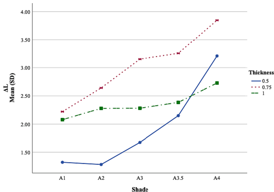
Fig. 3. Delta L values across all background tooth shades (line graph).
