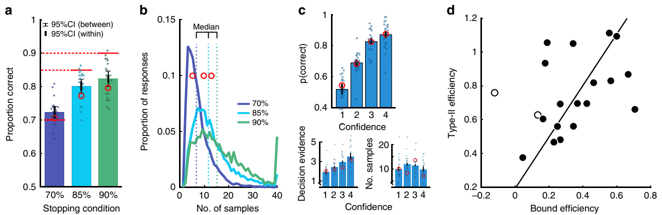
Fig. 3 The relationship between Type-I bound efficiency and Type-II efficiency. a Average proportion correct in each condition of the Stopping task. The horizontal red lines subtend the target performance level in each condition. Error bars show 95% within-subjects (thick) and between-subjects (thin) confidence intervals n = 20 . The red circles show the predicted performance based on the fitted parameters of the model. b Average proportion of trials by the number of samples the observers chose to respond to in each condition of the Stopping task. Vertical dashed lines show the average median number of samples. Red circles show the predicted median number of samples based on the fitted parameters of the model. c Proportion correct (top), decision evidence (bottom left) and number of samples (bottom right) by confidence rating in the Replay task. Error bars show 95% within-subjects confidence intervals ( n = 20 ), and red circles show the predicted performance at each confidence level based on the fitted parameters of the model. d Each observer's bound efficiency ( x -axis) by their Type-II efficiency ( y -axis) and the line minimising the perpendicular distance from these points, here shown excluding two outlier participants (open circles) whose optimal bound was estimated using maximum performance rather than 85% correct ( y = 1.5x + 0.2 , p -value for slope = 0.026, one-sided, based on bootstrapping, with outlier participants removed).
