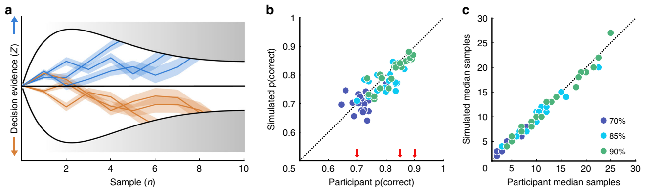
Fig. 2 Computational model and simulations. a On each trial, the observer sums the decision evidence ( z ) of each sample, n , which is the log-probability of the orientation, given the distribution ( \ell_n ), corrupted by additive i.i.d. Gaussian noise ( \epsilon_n , with standard deviation \sigma ), and weighted according to the observer's leak ( v_n , an exponential function of \alpha ). Three example trials are shown from each distribution (blue and orange traces, with the shading representing the variability due to noise). Evidence accumulation stops once the evidence reaches the bound, in this case a collapsing bound defined by \Lambda_n , shown by the black curves. b Participant proportion correct against the simulated data based on the fitted parameters of the computational model, for each participant in each condition of the Stopping task (70%, 85% and 90% correct in blue, cyan and green, respectively). The diagonal shows equality. Red arrows mark the performance targets. c The same as b for the median number of samples the observer chose to respond to.
