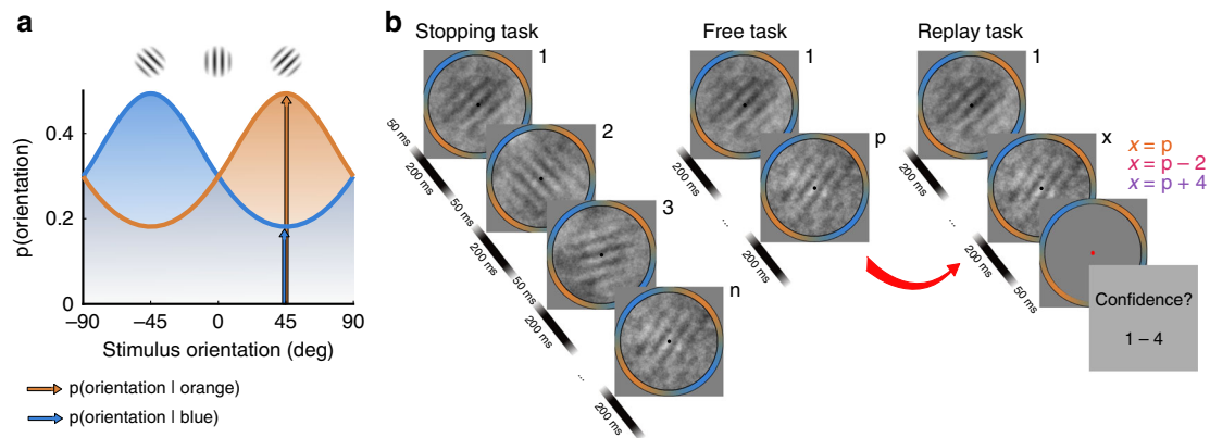
Fig. 1 Procedure. On each trial, observers were shown a series of oriented Gabors and had to determine which distribution the orientations were drawn from. a The orientations were drawn from one of two circular Gaussian (von-Mises) distributions centred on -45^\circ (blue) and +45^\circ (orange) relative to vertical ( 0^\circ ). The distributions were overlapping such that a stimulus oriented 45^\circ from vertical is most likely to have been drawn from the orange distribution (orange arrow) but still could have been drawn from the blue distribution (blue arrow). b The experiment involved two sessions. In session 1, observers completed the Stopping task. On each trial of the Stopping task the series of stimuli continued until observers entered a Type-I response: blue or orange distribution. They were asked to enter their response when they felt they had a certain probability of being correct. The three target performance levels (70%, 85% and 90% correct) were completed in separate blocks. In session 2, observers completed the Free task followed by the Replay task. The Free task was the same as the Stopping task, except observers were asked to enter their response when they felt ready (after p samples). In the Replay task, observers entered their Type-I response once cued (fixation changing to red). They then gave a Type-II response: a rating (1 to 4) of how confident they were that they were correct. Unbeknownst to observers, the Replay task actually replayed the exact same trials from the Free task, except the number of samples was either the same as they had chosen to respond to ( x = p ), two fewer ( x = p - 2 ), or four additional samples ( x = p + 4 ). These trials comprise the Same, Less and More conditions, respectively. Across all tasks, the fixation point (black dot) and colour guide were present throughout each trial. The samples were presented at a rate of 4 Hz, with 200 ms of stimulus presence (including 25 ms ramp at onset and offset) and 50 ms inter-stimulus interval. All tasks consisted of repetitions of the same 100 trials pre-defined for each observer.
