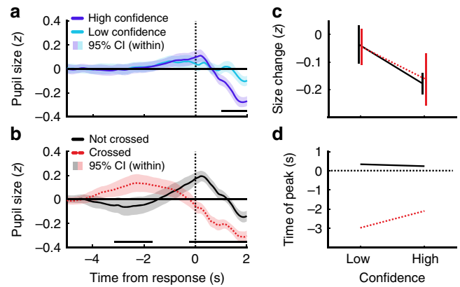
Fig. 6 Pupil response to confidence and boundary crossing. Average standardised pupil size in the Replay task across response-aligned (dashed vertical black line) time-windows, baselined to the average over -5 to -4 s. Shaded error bars show the 95% within-subjects confidence intervals. Differences between these lines were assessed using Wilcoxon sign rank tests, with significant clusters shown in the horizontal lines at the bottom of each plot. a Trials separated by confidence rating (high = 3 and 4, low = 1 and 2), with the black horizontal line showing significant differences. b Trials separated by whether it was likely that the observer's covert bound was crossed, based on the fitted parameters of the computational model, with the black horizontal line showing significant differences. c Average change in pupil size from the time of the response to 1 s after the response for low- and high-confidence trials within crossed (red dashed) and not crossed (black) trials. Error bars show 95% within-subjects CI. d Time of peak pupil size in the low- and high-confidence trials within crossed (red dashed) and not crossed (black) trials.
