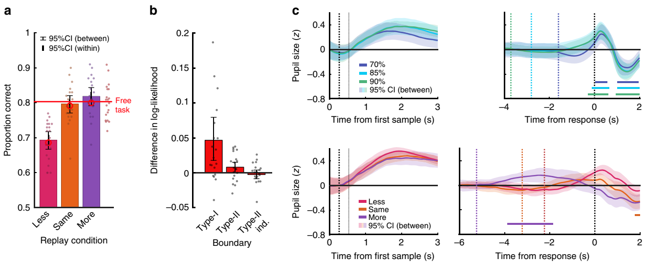
Fig. 4 Evidence for a covert bound on Type-I evidence accumulation. a Average proportion correct in each condition of the Replay task. In the Same condition (orange), observers were shown the same number of samples as they had chosen to respond to in the Free task, in the Less condition (magenta) they were shown two fewer samples, and in the More condition (purple), four additional samples. The red horizontal line shows the average proportion correct in the Free task, where the exact same trials were shown (with the exception of the condition manipulation). Error bars show 95% within-subject (thick) and between-subject (thin) confidence intervals ( n = 20 ). Open red circles show the model predictions based on simulations of the bounded model. b Difference in log-likelihood (relative improvement in fit) between the model fit with a covert boundary compared to the model without. The bars show the improvement in the fit to Type-I responses with a bound on Type-I evidence accumulation (labelled Type-I), the improvement in the fit to Type-II responses when the Type-II is bounded at the same time as the Type-I evidence (labelled Type-II), and the improvement in the fit to Type-II responses when an independent bound is fit to the accumulation of Type-II evidence (labelled Type-II ind.). Error bars show 95% between-subject confidence intervals n = 20 . c Standardised pupil size in the Stopping task (top) and Replay task (bottom), averaged across time-windows aligned to the start of each trial (left) and to the response (right). Shading shows 95% between-subjects confidence intervals ( n = 19 ). Trial-start aligned data were baselined to the average at time 0, response-aligned data were baselined to the average prior to trial start ( -4 to -3 s in the Stopping task, and -6 to -5 s in the Replay task). Black vertical lines in the trial-start plots show the timing of the 2nd and 3rd samples. Vertical lines in the response plots show the average median timing of the start of the trial. Differences from baseline in the response-aligned epochs were tested using two-sided Wilcoxon sign rank tests, with significant clusters shown with horizontal lines (corrected p < 0.05 ).
