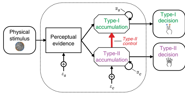
Fig. 5 The accumulation of evidence for Type-I and Type-II decisions. The dashed box encloses the hidden decision processes, which determine the relationship between the observable variables (the physical input and behavioural output). Information from the physical stimulus is transformed into decision evidence, which is accumulated for the Type-I decision with additive Gaussian noise ( \epsilon_s ) and weighted according to the leak ( \alpha_s ). Evidence accumulated for the Type-II decision incurs additional noise ( \epsilon_c ) and a separate leak ( \alpha_c ). Type-II control is exerted on the Type-I evidence accumulation process, depicted by the red arrow, where the accumulated evidence is sent to the decision output once the boundary is reached, based on the Type-II evidence. The Type-II evidence may continue to accumulate even after the boundary has been reached.
