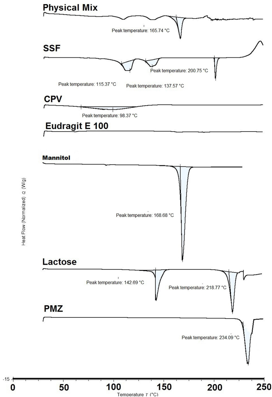
Fig. 5. Differential scanning calorimetric scans of untreated promethazine (PMZ), lactose, mannitol, Eudragit E 100, crospovidone (CPV), sodium stearyl fumarate (SSF) and their physical mixture.
