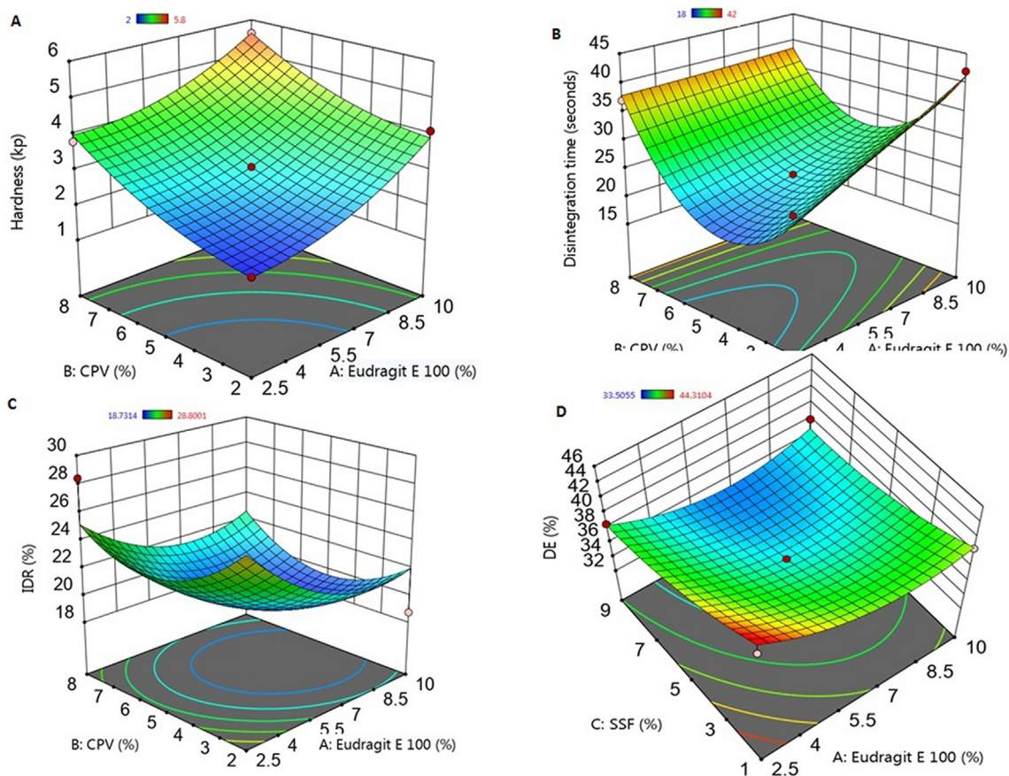
Fig. 2. Response surface plots for the effect of independent variables on promethazine (PMZ) tablet hardness (A), disintegration time (B), Immediate dissolution rate (IDR) (C) and dissolution efficiency (DE) (D). The plot highlights the interactive effect of two factors on the response when the third factor is maintained at its middle range.
