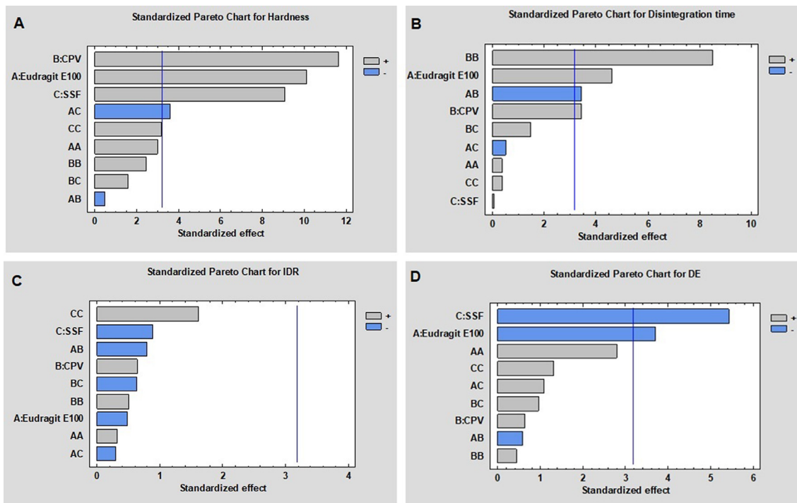
Fig. 1. Standardized Pareto chart for the effect of independent variables on promethazine (PMZ) sublingual tablet hardness (A), disintegration time (B), Immediate dissolution rate (IDR) (C) and dissolution efficiency (DE) (D).
