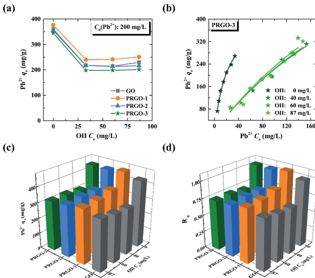
Fig. 8 Co-adsorption of Pb^{2+} in the presence of OII. (a) The equilibrium adsorption capacities of Pb^{2+} on GO and PRGO as a function of OII concentration. (b) The adsorption isotherms of Pb^{2+} on PRGO-3 under different OII concentration. The solid lines are the Langmuir model simulations. (c) The maximum adsorption capacities of Pb^{2+} on GO and PRGO in the presence of OII. (d) The corresponding ratios R_q of Pb^{2+} on GO and PRGO in the presence of OII.
