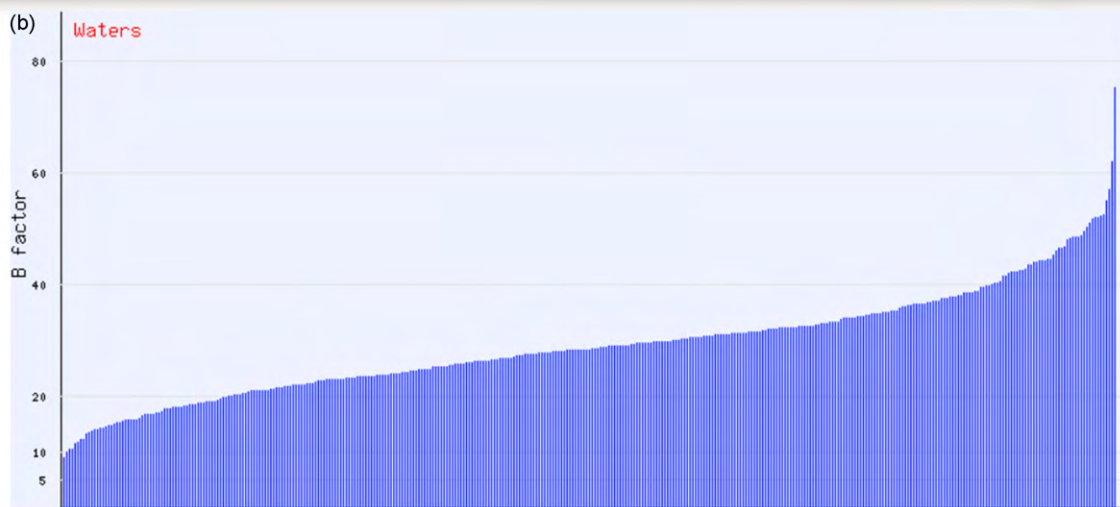
Fig. 11. Access to EDBase for VZ93 example. (a) Four models (with goodness-of-fit indicators) are stored in the database and (b) solvent B-factor distribution after refinement.
