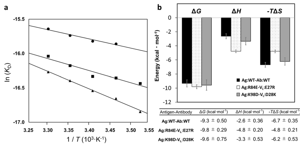
Figure 4. Comparison of thermodynamic profile of antigen-antibody interactions. (a) Plots of \ln(K_D) vs 1/T ( \text{K}^{-1} ) for wild-type antigen-antibody ( \bullet ), Ag:R84E- V_L :E27R ( \blacktriangle ), and Ag:K98D- V_L :D28K ( \blacksquare ). (b) Bar graphs of the equilibrium thermodynamic parameters obtained from van't Hoff analyses. Error bars correspond to the standard deviation. The standard deviations of \Delta H and -T\Delta S were calculated from the fitting data, respectively, and that of \Delta G was calculated from \Delta G = \Delta H - T\Delta S with error propagation. Values are reported at 298 K.
