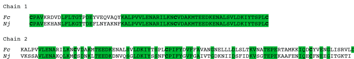
Figure 1. Sequence alignment of Felis catus (Fc) dander allergen Fel d1 and Nycticebus javanicus (Nj) brachial gland secretion protein. Identical residues are shaded in grey.
