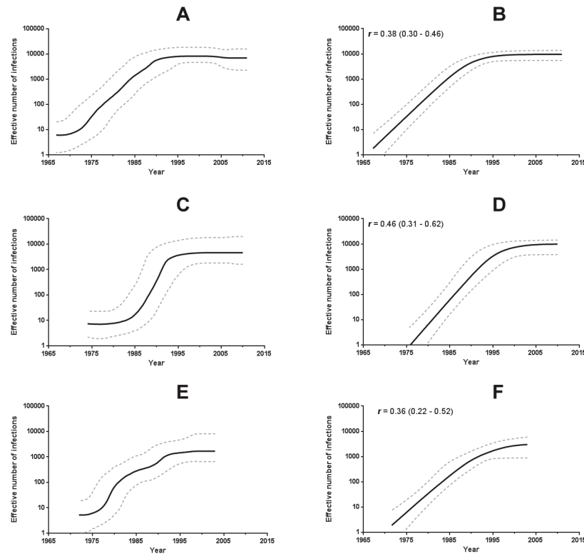
Figure 6. Demographic history of the HIV-1 B_{CAR} (A, B), B_{CAR-JM} (C, D), and B_{CAR-TT} (E, F) clades circulating in Hispaniola, Jamaica and Trinidad and Tobago, respectively. Effective number of infections (y-axis; log 10 scale) through time (x-axis; calendar years) estimated using Bayesian skyline (A, C, E) and logistic (B, D, F) growth coalescent model. Median estimates of the effective number of infections (solid line) and 95% HPD intervals of the estimates (dashed lines) are shown in each graphic. The median growth rate (with the corresponding 95% credibility interval in parenthesis) of each clade estimated under logistic growth model is indicated in the upper left corner. doi:10.1371/journal.pone.0106045.g006
