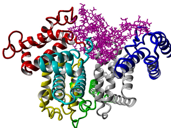
Figure 2. Structure of human serum albumin with different coloring for the different HSA subdomains: IA—red; IB—cyan; IIA—yellow; IIB—green; IIIA—grey; IIIB—blue. Hyaluronate is colored pink. The figure represents one of many structures of the HAS–hyaluronate complex. This particular complex is referred to as complex number 1 in Table 1.
