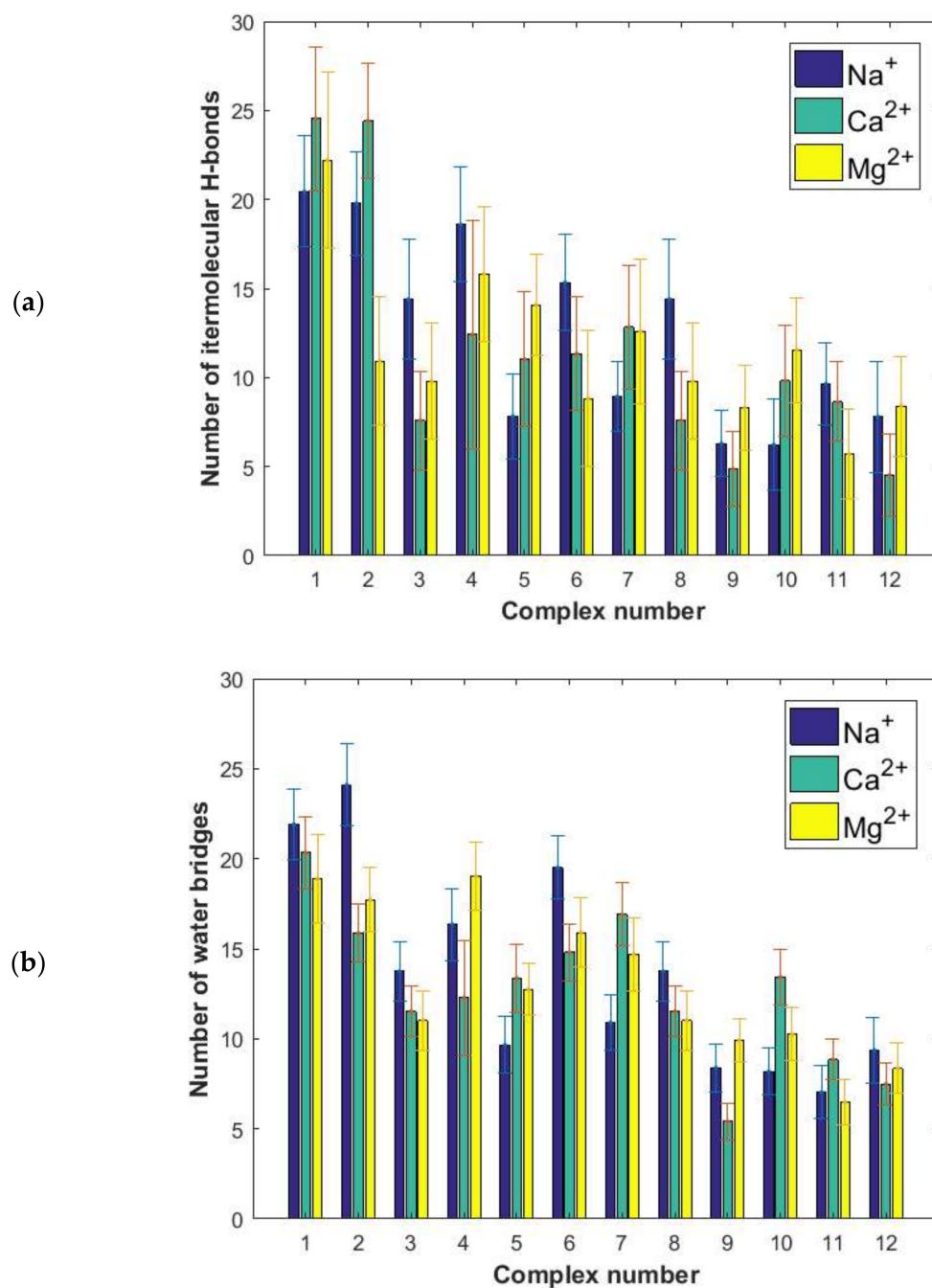
Figure 5. (a) Number of direct intermolecular H-bonds. (b) Water bridges between HSA and HA for different complexes evaluated by MD.
