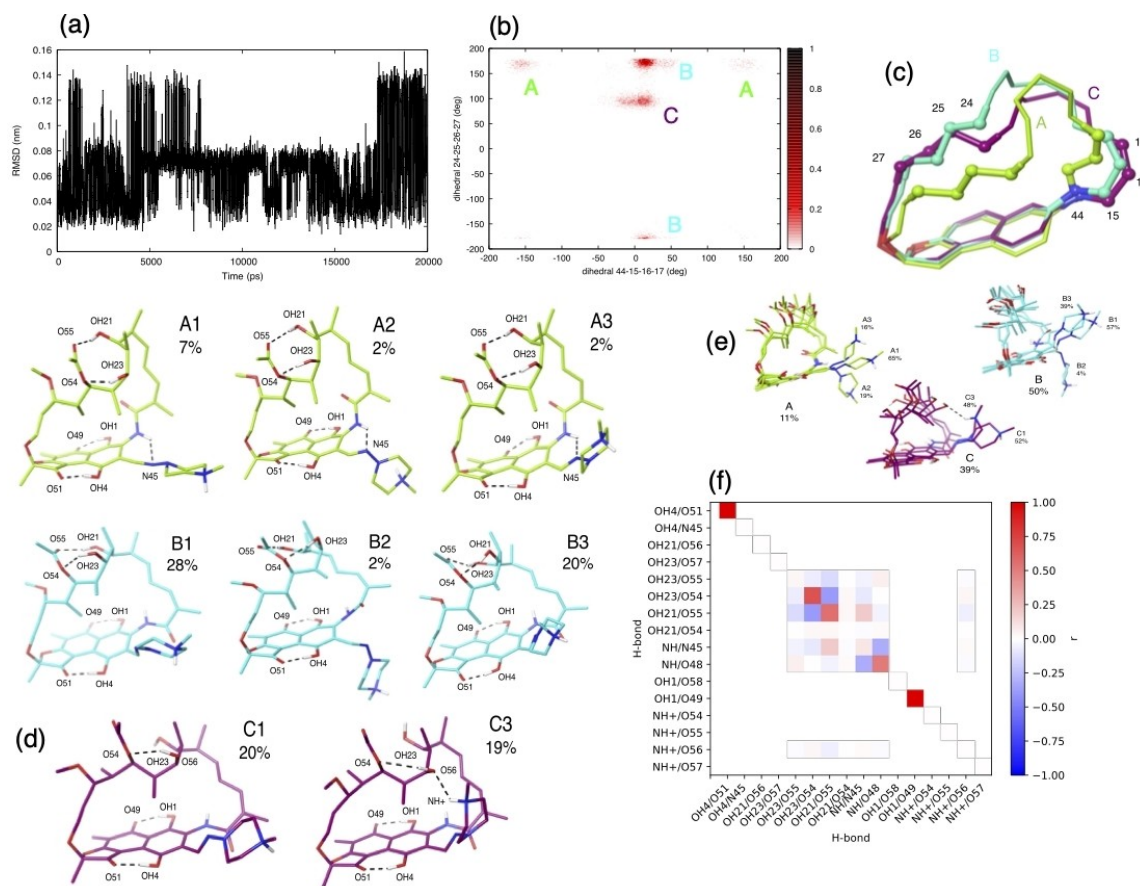
Figure 7. The results of the simulation of zwitterionic rifampicin in D2O. (a) The time course of the RMSD to the crystallographic structure shows fluctuations between at least three conformations. (b) The distribution associated with two dihedrals of the macrocycles of the three clusters. (d) The result of the clustering analysis. (e) The comparison between sub-clusters. (f) the formation probability (on the diagonal) and the correlation (off-diagonal) between hydrogen bonds; all pairs of hydrogen bonds that are able to form are considered.
