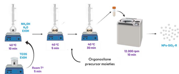
Scheme 1 Stöber method scheme and conditions used for nanoparticles synthesis and functionalization.
