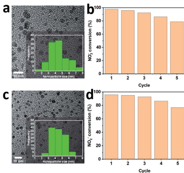
Fig. 7 (a) TEM image of peptide-directed Pd-on-Au NP 100 sc% after five catalytic cycles. (b) Nitrite conversion for Pd-on-Au NP in five cycles. (c) TEM image of peptide-directed \text{Pd}_{26}\text{Au}_{74} NP after five catalytic cycles. (d) Nitrite conversion for \text{Pd}_{26}\text{Au}_{74} NP in five cycles (inset is the size distribution plot). Reaction condition: \text{NaNO}_2 ( 40 \text{ mg L}^{-1} ), \text{H}_2 and \text{CO}_2 ( 50 \text{ mL min}^{-1} ), catalyst ( 400 \text{ mg L}^{-1} of Pd), \text{H}_2\text{O} ( 100 \text{ mL} ), 600 rpm, 1 atm pressure, 75 min.
