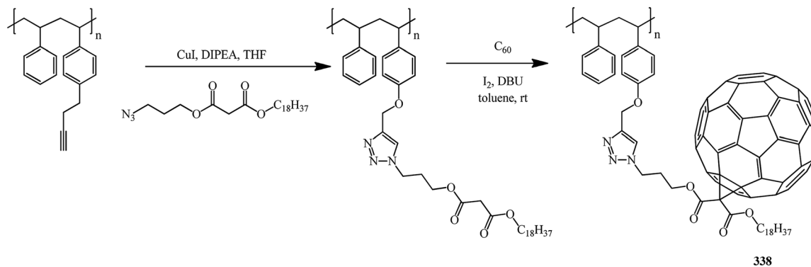
Scheme 93
