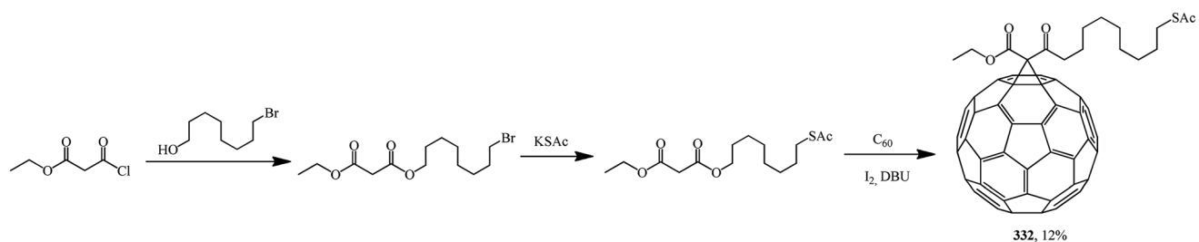
Scheme 89
