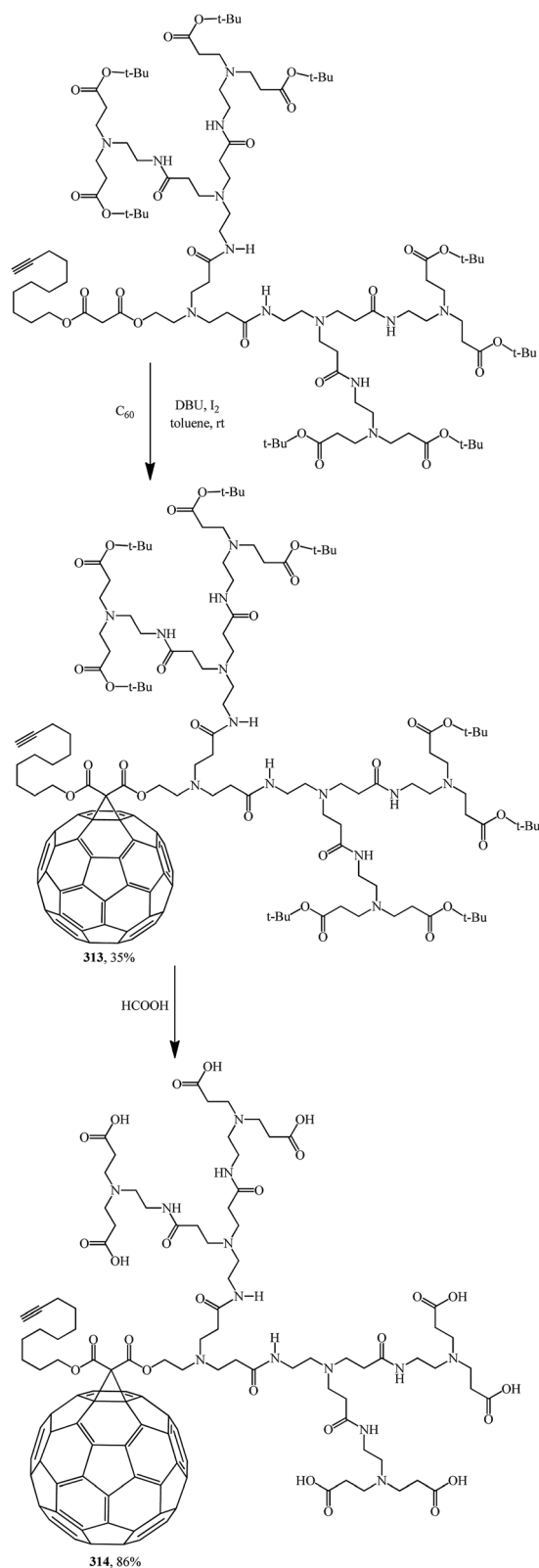
Scheme 87
