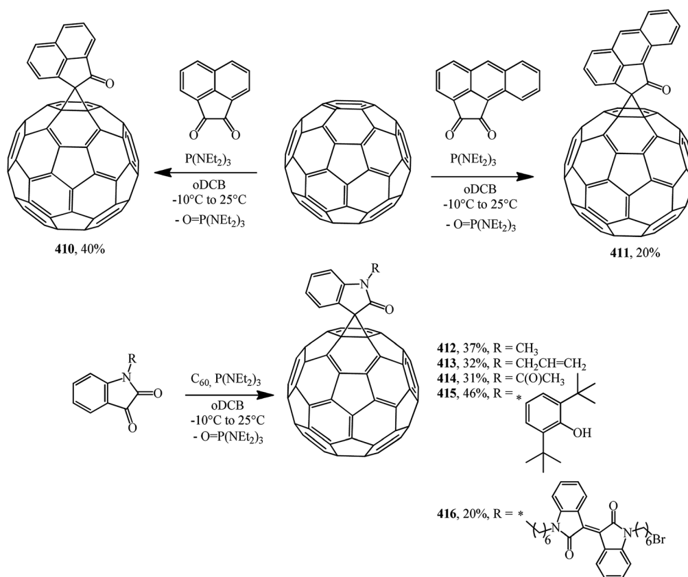
Scheme 107
