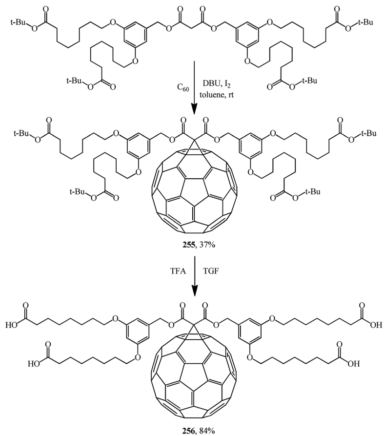
Scheme 72
