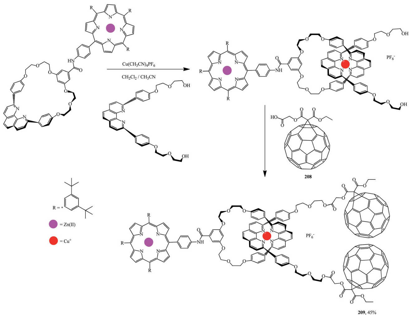
Scheme 56
