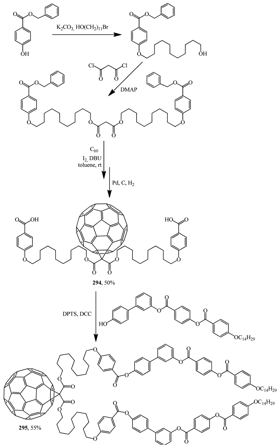
Scheme 80
