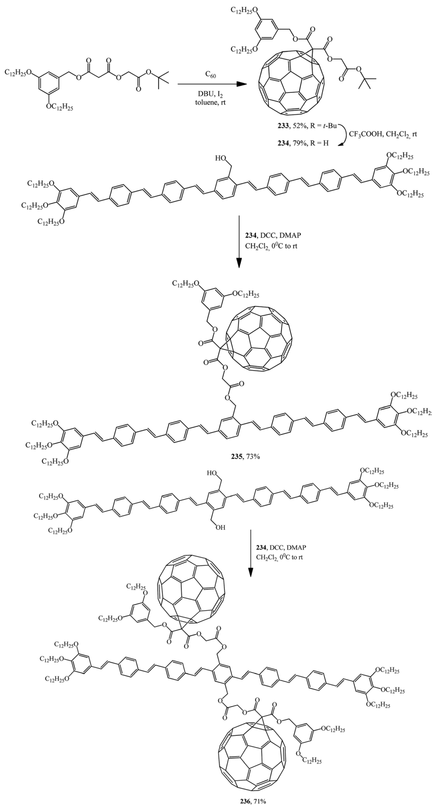
Scheme 65
