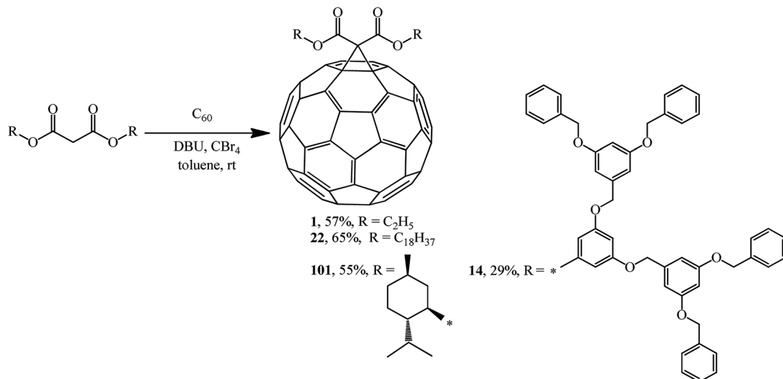
Scheme 37
