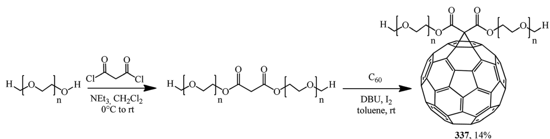
Scheme 92
