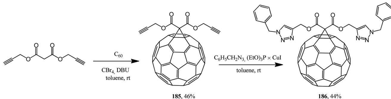
Scheme 47
