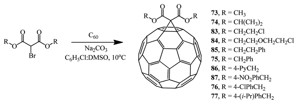
Scheme 33
