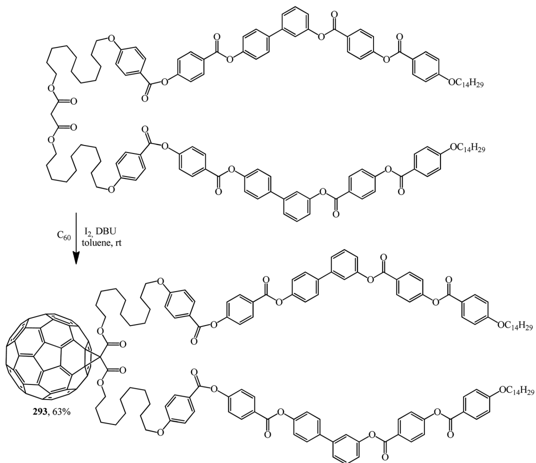
Scheme 79
