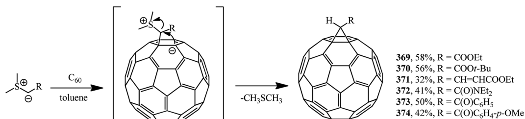
Scheme 101
