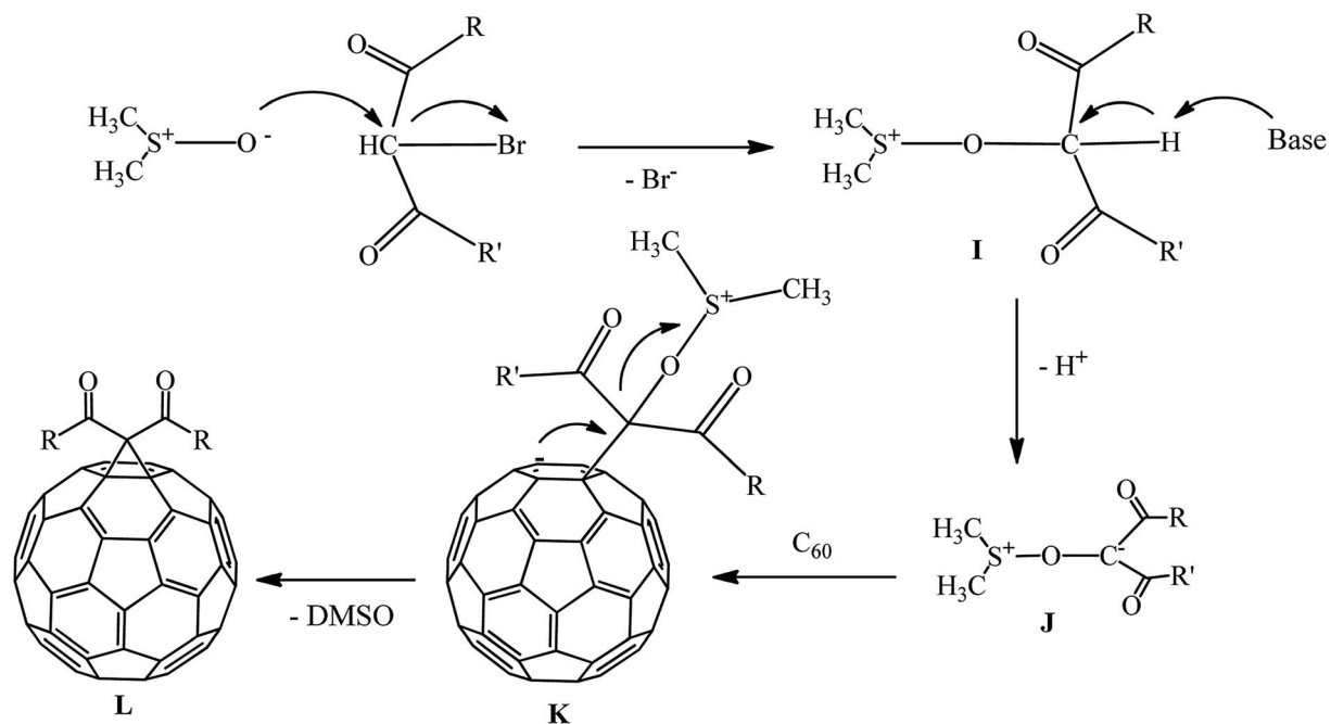
Scheme 36
