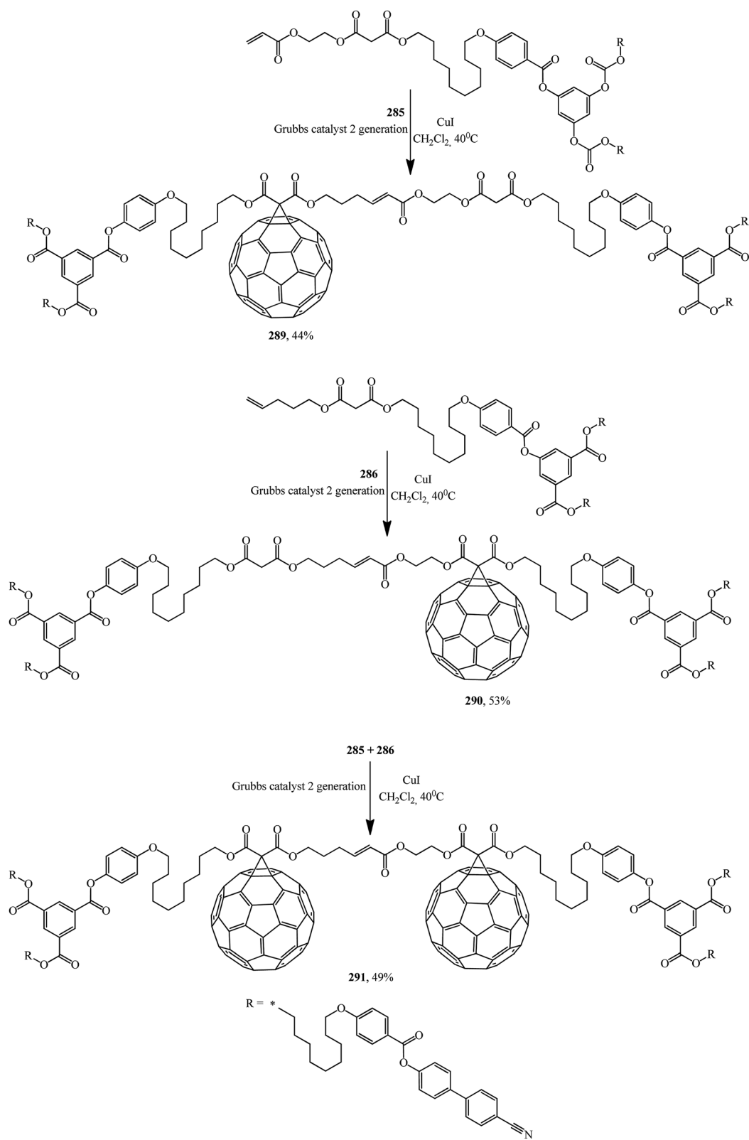
Scheme 77
