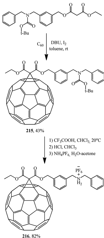
Scheme 58
