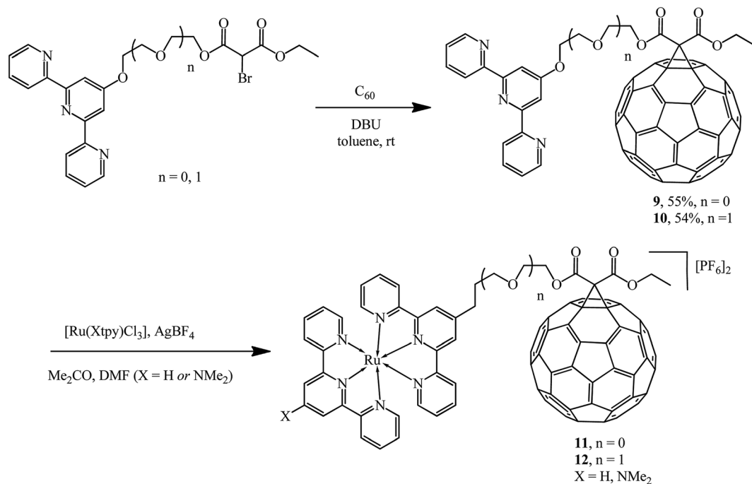
Scheme 6
