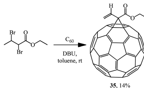
Scheme 11
