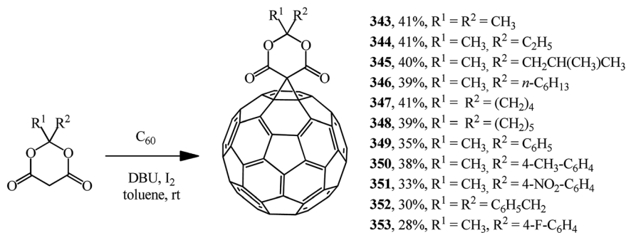
Scheme 96
