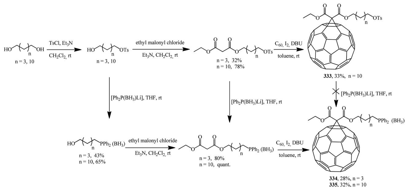
Scheme 90
