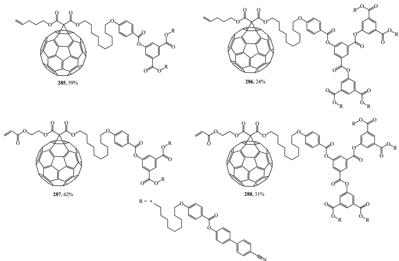
Fig. 21 Fullerene-containing dendrimers 285–288.
