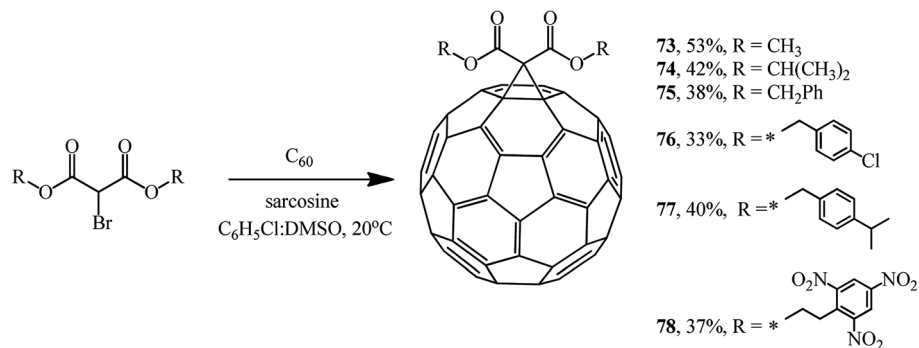
Scheme 28
