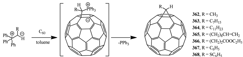
Scheme 100
