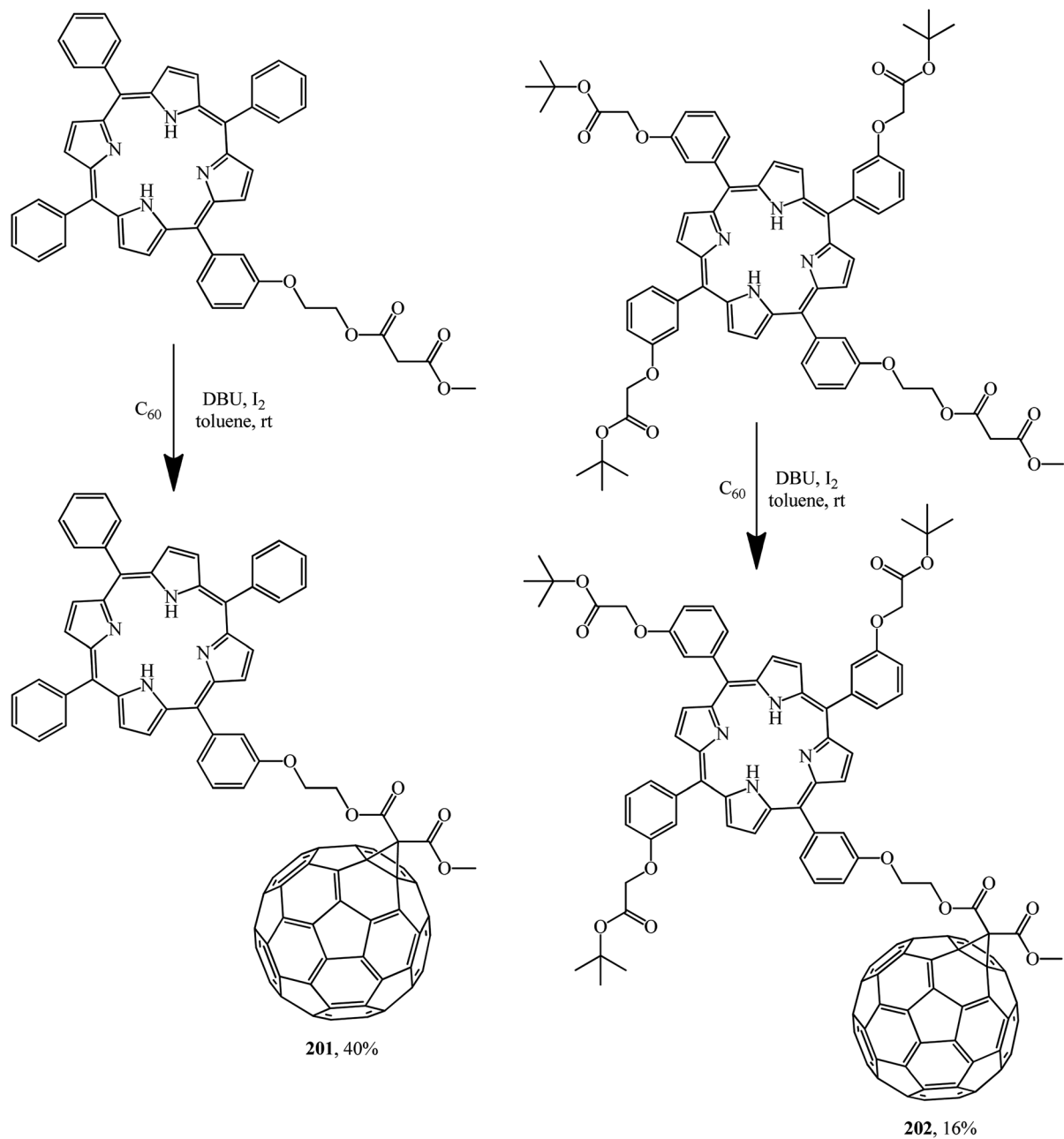
Scheme 53
