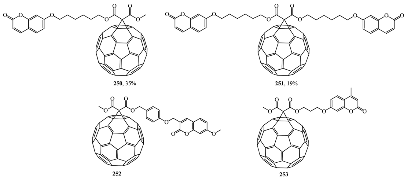
Fig. 14 Fullerene–coumarin diads 250–253.
