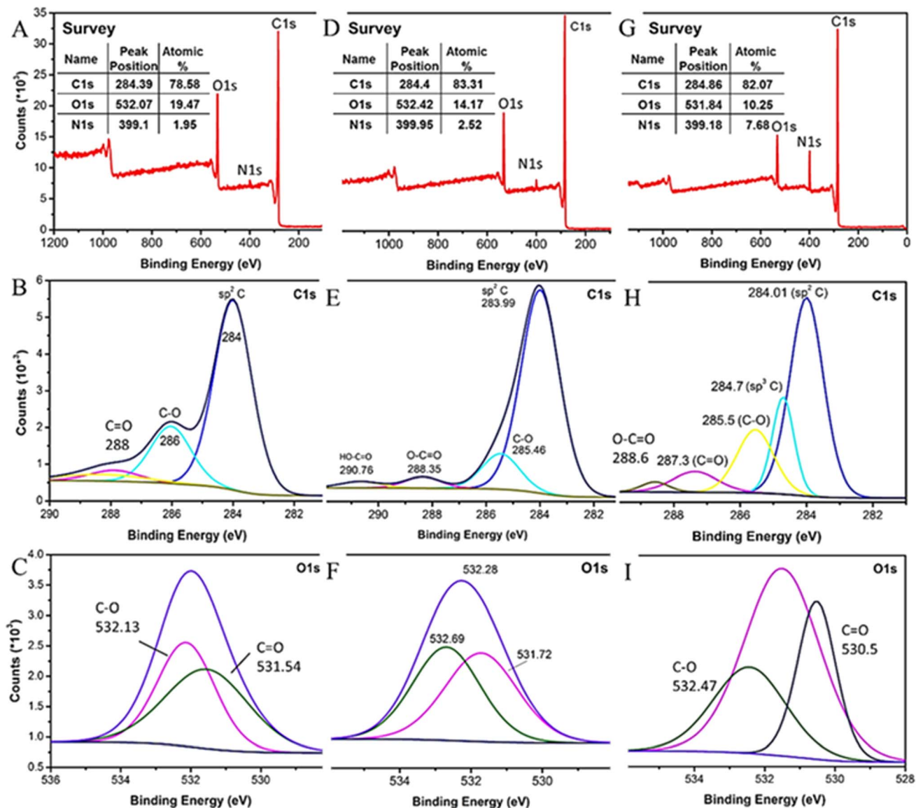
Fig. 4 XPS spectra of [A–C] reduced graphene oxide, [D–F] hyperbranched polyester, and [G–I] in situ modified RGO.
