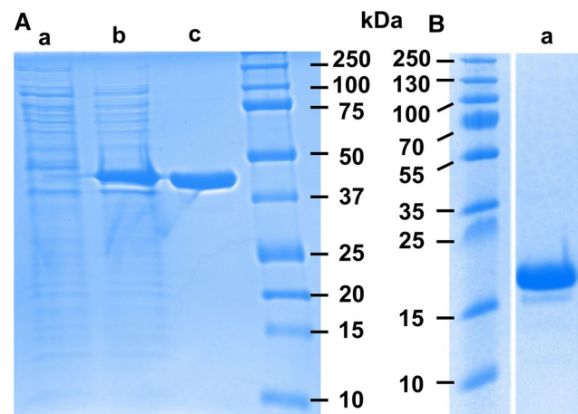
Fig. 3 SDS-PAGE results for the expression and purification of matchout labelled protein. A Maltose binding protein (MBP). a Uninduced cellular extract; b extract from induced cells; c purified MBP after immobilized metal ion affinity chromatography. B SCR-19/20 from CFH. a After cation exchange and size exclusion chromatography
