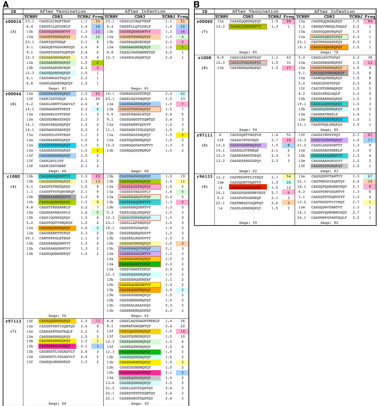
Figure 2. Clonotypic architecture of CM9-specific CD8 + T cell populations. TCRB CDR3 amino acid sequences, TCRBV and TCRBJ usage, and the relative frequency of CD8 + T cell clonotypes specific for the CM9 epitope are shown for all eight macaques at week 2 after vaccination with Ad5 (left) and at week 4 after infection with SIVmac239 (right). The number of challenges required for infection to occur is indicated in each case underneath the individual macaque identification codes. Data are separated according to macaques with the lowest (A) and highest (B) set point pVL values. Colored boxes in the frequency column (percentages) indicate clonotypes within individual macaques that have the same TCRB CDR3 amino acid sequence at both time points shown; colored boxes in the CDR3 sequence column indicate public clonotypes. Public clonotypes were defined on the basis of TCRB amino acid sequences that were present in more than one macaque; TCRB sequences reported both in this study and in a previous study were included in the analysis (reference 17). The corresponding TCRB CDR3 nucleotide sequences are shown in Table 1.
