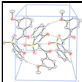
Fig. 2. Unit cell packing of (I) showing non-classical hydrogen bonding interactions with dashed lines; H atoms not involved in H-bonds have been excluded for clarity.
