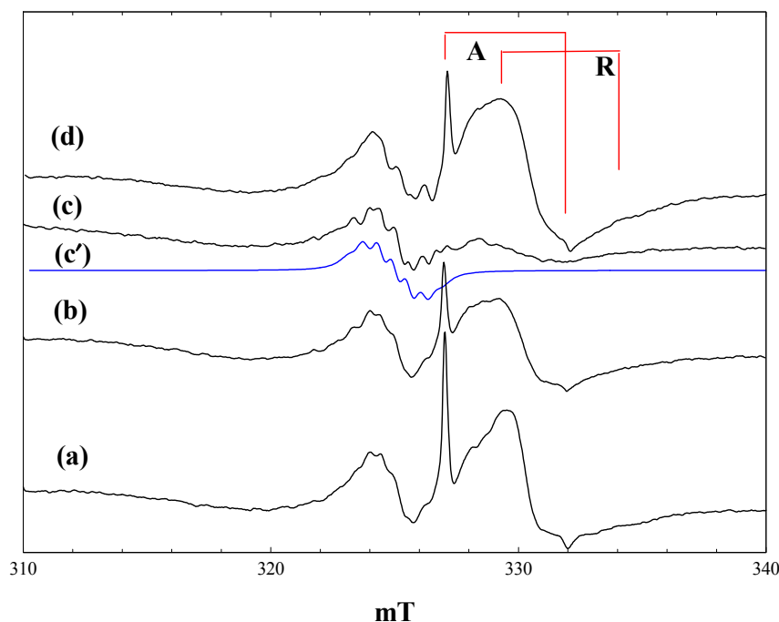
Figure 3. EPR spectra of P25 titania in a solution of phenoxyacetic acid in acetonitrile at 4 K. (a), During irradiation with low intensity 400 nm light; (b), During irradiation with high intensity 400 nm light; (c), during irradiation with high intensity broad band light; (d), after stopping irradiation; (c'), a simulated spectrum of the phenoxyacetic acid radical cation, as described in the text.
