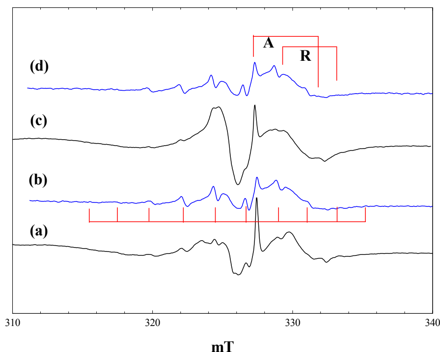
Figure 6. EPR spectra of P25 titania in an equimolar mixture of maleimide and pivalic acid in acetonitrile. (a), During irradiation with high intensity 400 nm light at 4 K; (b), during irradiation with high intensity 400-nm light at 80 K; (c), after irradiation with high intensity broad-band light at 4 K; (d), after irradiation with high intensity broad band light at 80 K.
