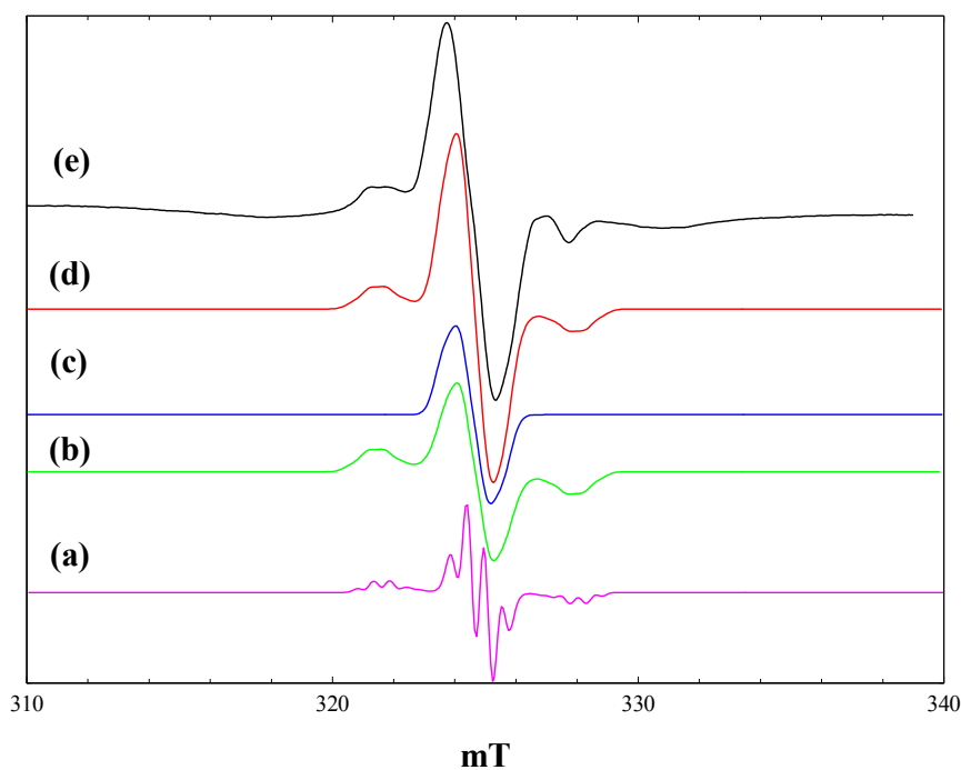
Figure 8. Simulation of the observed spectrum obtained during irradiation of P25 titania in an equimolar mixture of maleimide and phenoxyacetic acid in acetonitrile with high intensity broad-band light at 4 K. (a), Simulation of the phenoxymethyl radical using the parameters described in the text and Gaussian line widths of 0.3 mT (parallel) and 0.5 mT (perpendicular); (b), Gaussian line widths of 0.5 mT (parallel) and 1.0 mT (perpendicular); (c), simulation of the maleimide radical anion (from Figure 5, b); (d), Sum of b and c; (e), observed spectrum.
