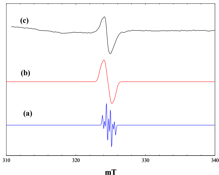
Figure 5. Comparison of simulated and observed spectra of the maleimide radical anion. (a), Simulated with a(\text{N}) = 0.262 mT, a(2\text{H}) = 0.580 mT, a(\text{NH}) = 0.031 mT, Gaussian line width of 0.2 mT; (b), Gaussian line width of 0.6 mT; (c), observed spectrum following broad-band irradiation at 80 K.
