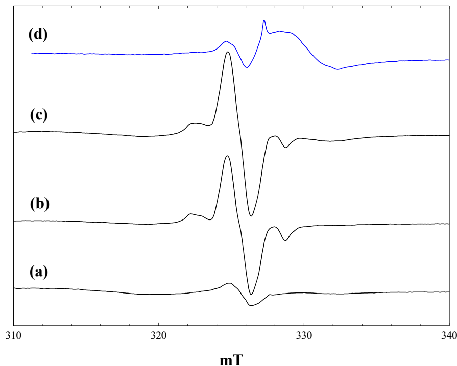
Figure 7. EPR spectra of P25 titania in an equimolar mixture of maleimide and phenoxyacetic acid in acetonitrile. (a), during irradiation with high intensity 400 nm light at 4 K; (b), during irradiation with high intensity broad band light at 4 K; (c), after irradiation with high intensity broad band light at 4 K; (d), after irradiation with high intensity broad band light at 80 K.
