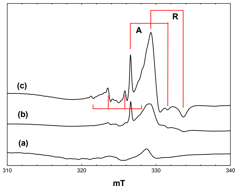
Figure 1. EPR spectra of P25 titania in acetonitrile at 4 K. (a), Prior to irradiation; (b), during irradiation with high intensity broad-band light; (c), after stopping irradiation.
