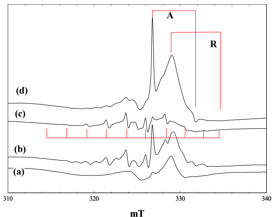
Figure 2. EPR spectra of P25 titania in a solution of pivalic acid in acetonitrile at 4 K. (a), During irradiation with low intensity 400 nm light; (b), during irradiation with high intensity 400 nm light; (c), during irradiation with high intensity broad band light; (d), after stopping irradiation.
