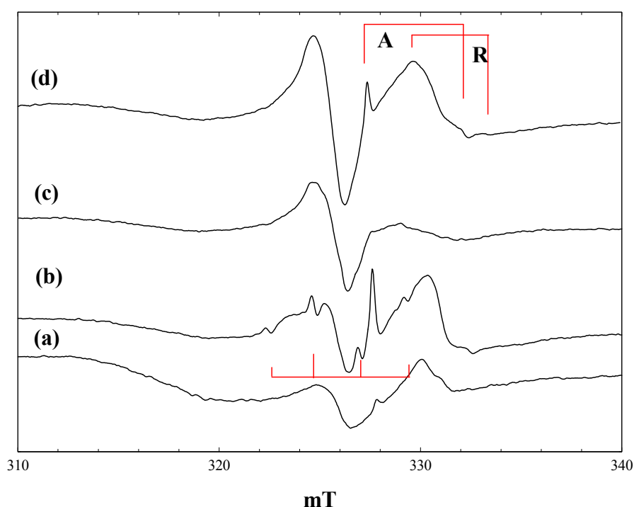
Figure 4. EPR spectra of P25 titania in a solution of maleimide in acetonitrile at 4 K. (a), During irradiation with low intensity 400 nm light; (b), during irradiation with high intensity 400 nm light; (c), during irradiation with high intensity broad band light; (d), after stopping irradiation.
