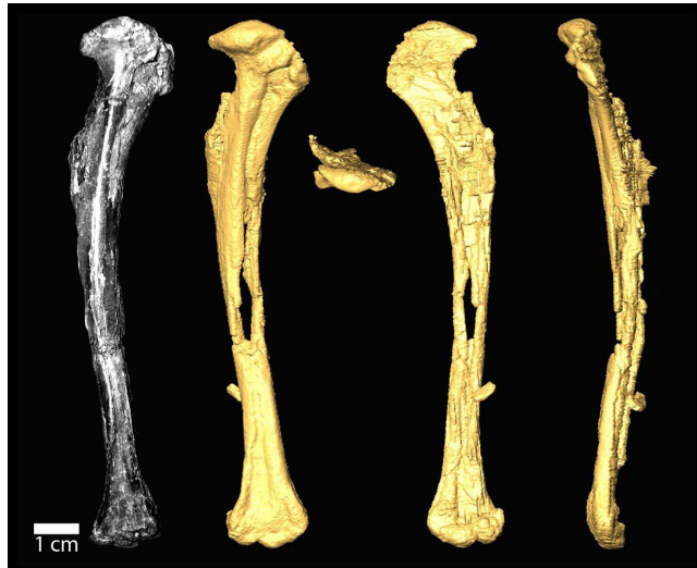
Figure 3. The holotype specimen of Tingmiatornis arctica , NUFV 1960, a complete left humerus. Photograph (left) and x-ray computed tomography images (right) of the element in caudal, proximal, cranial, and ventral views.
