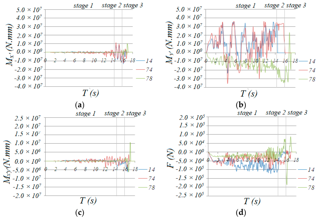
Figure 13. Time history of internal forces of traverse bar 14, 78 and 74: (a) M_{x'} , (b) M_{y'} , (c) M_{x'y'} , (d) F .
