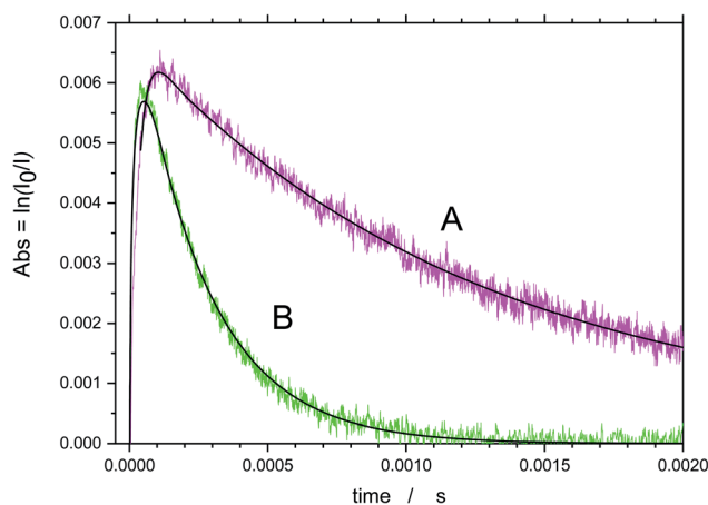
Fig. 4 Sample transient absorption signals of OH in O 3 /O 2 /H 2 /He mixture. A – without TMP, B – [TMP] = 3.6 × 10 14 molecule per cm 3 . Longer rise time (compared with the profiles where water was used) is apparent.
